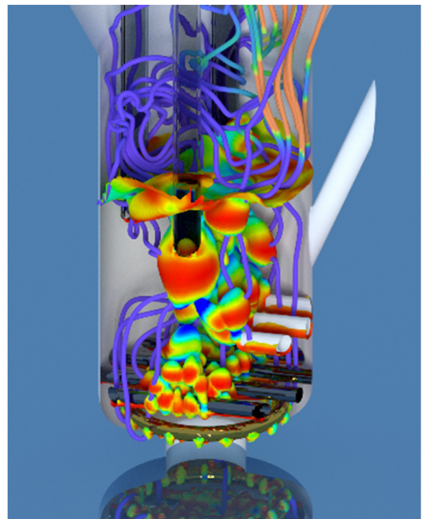
Figure 4. Researchers at the Idaho Nuclear Technology and Engineering Center at the Idaho National Laboratory are using simulations to better understand how well the waste and bed material mix, and how mixing in the vessel affects the performance.
