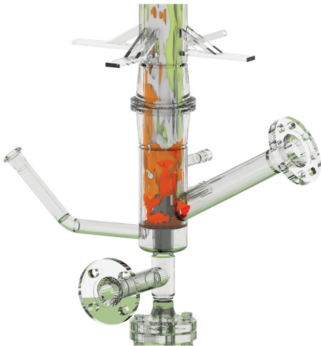
Figure 3. Gasification technology modeling using the multiphase CFD software portfolio.
