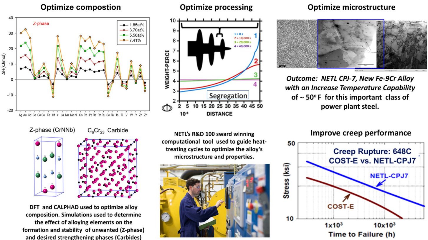
Figure 1. The alloy development process can be optimized through computational science.
