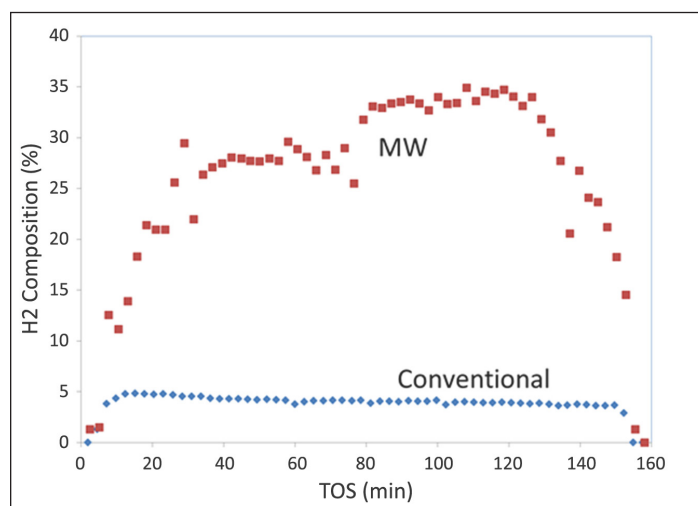
FIGURE 4: Coal steam gasification.
