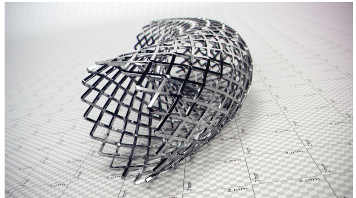
Figure 1. An NETL/Boston Scientific-developed platinum/chromium alloy is highly x-ray visible and has an improved physical property for producing better human coronary stents.
