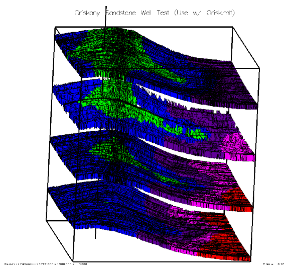
Figure 6. Reservoir simulation output shows pressures in four layers of a naturally fractured and folded sandstone. Simulation of the injection of carbon dioxide for storage.
