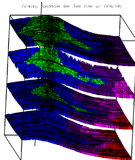
Figure 6. Reservoir simulation output shows pressures in four layers of a naturally fractured and folded sandstone. Simulation of the injection of carbon dioxide for storage.
