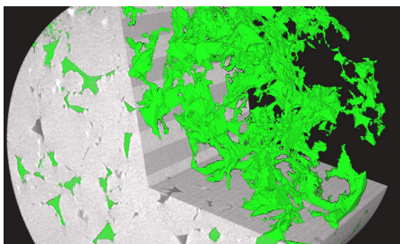
Figure 5. NETL's CT scanners are used to image geomaterials and understand interactions with fluids. Two examples—3D structures of CO 2 reacted zones in cement fractures, and pore space in reservoir rock—illustrate these capabilities.
