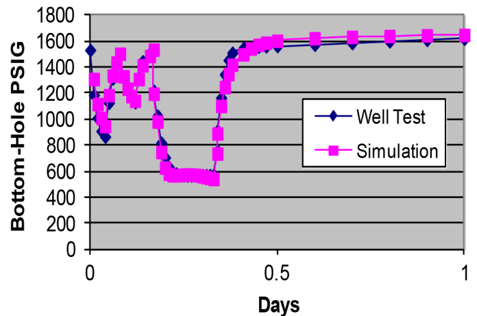
Figure 3. Measured and simulated wellhead pressure.
