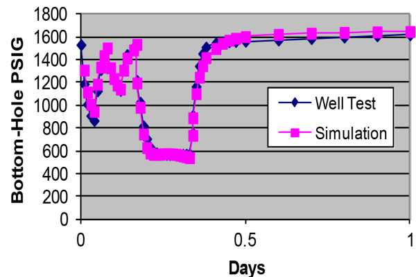
Figure 3. Measured and simulated wellhead pressure.
