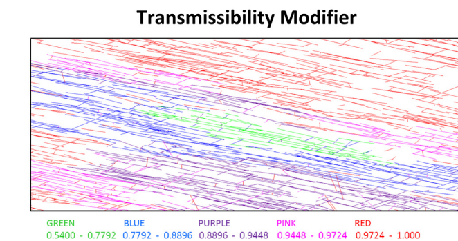
Figure 2. A snapshot after 20 days of gas production showing changes in fracture transmissibility due to induced geomechanical stresses acting on the fractures shown in Figure 1. The smaller the modifier, the smaller the fracture aperture compared to its initial size.
