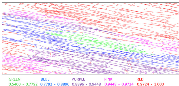
Figure 2. A snapshot after 20 days of gas production showing changes in fracture transmissibility due to induced geomechanical stresses acting on the fractures shown in Figure 1. The smaller the modifier, the smaller the fracture aperture compared to its initial size.
