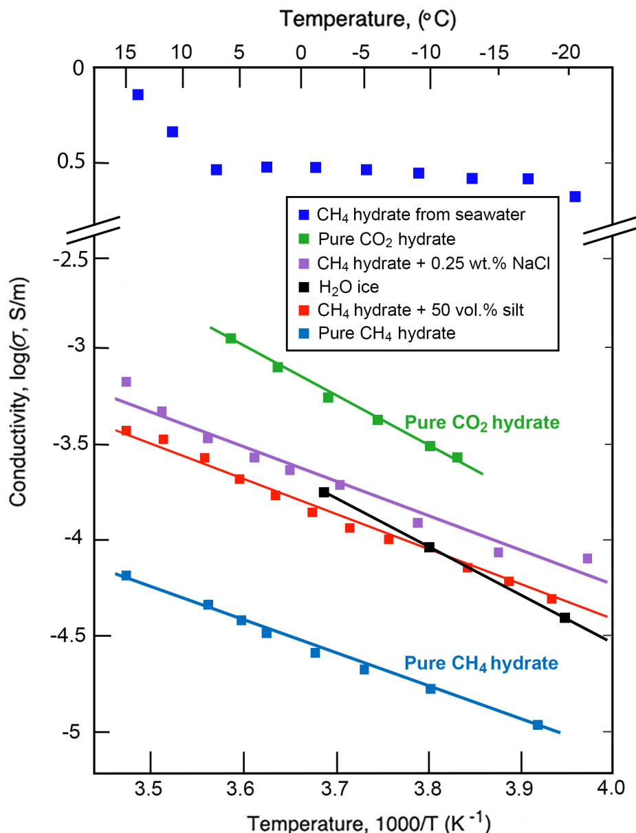
Figure 2. Electrical conductivity ( \sigma ) versus reciprocal temperature (Arrhenius) plot for pure \text{CO}_2 hydrate compared with our previous tests on ice, pure \text{CH}_4 hydrate, \text{CH}_4 hydrate with \text{SiO}_2 sediments (50 vol% silt shown here), \text{CH}_4 hydrate with 0.25 wt% NaCl, and \text{CH}_4 hydrate formed from flash-frozen seawater. \text{CO}_2 hydrate and all \text{CH}_4 hydrate samples other than the seawater sample were formed from the identical batch of seed ice. Amongst this group, \text{CO}_2 hydrate exhibits the highest conductivity. \text{CH}_4 hydrate prepared from seawater, however, is significantly more conductive than all other samples plotted here due to a coexisting brine component that formed and remained within that sample throughout testing. (Note break in vertical axis.)
