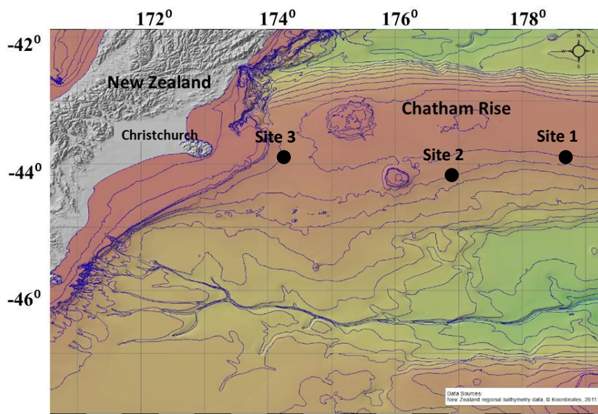
Figure 1: Coring locations during SO226/2 in February 2013 on the Chatham Rise, off the eastern coast of New Zealand.
