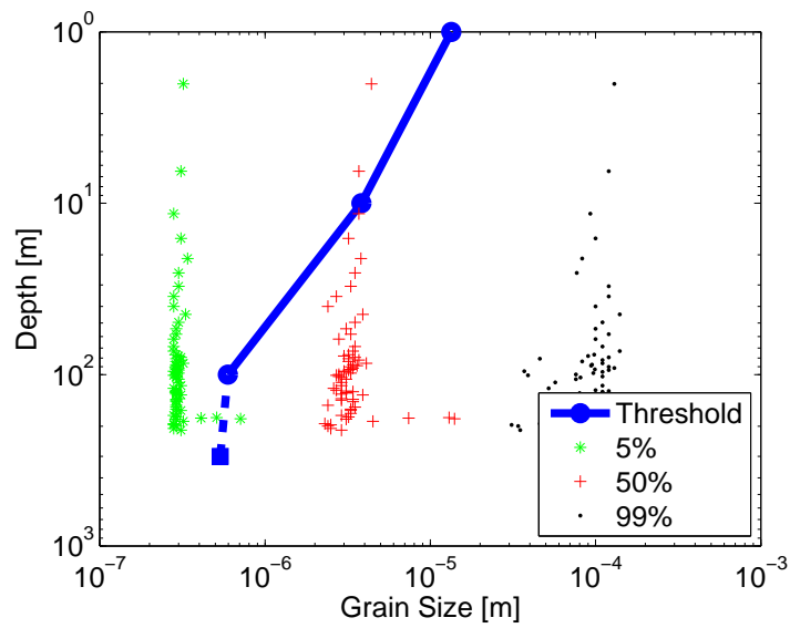
Figure 3-15: Grain-size distribution from site 1245b of southern Hydrate Ridge [30] overlaid on plot of threshold grain size between capillary invasion and fracture opening as a function of depth.
