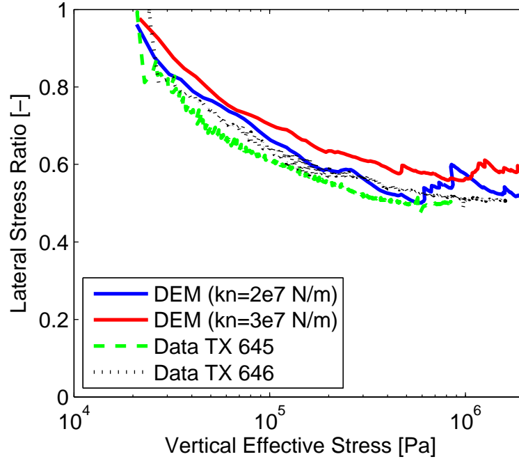
Figure 3-3: Experimental lateral-to-vertical stress ratio curves for sediments from Hydrate Ridge [93], and comparison with DEM simulations for the same values of grain stiffness used to match the vertical stress–strain behavior in Figure 3-2.
