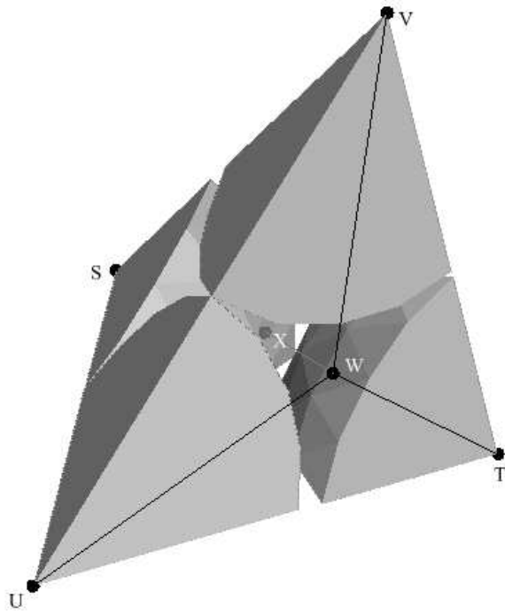
Figure 2-5: Representation of a pore throat in a three-dimensional grain-scale model [79]. The throat is the section with minimum cross-sectional area between two pore bodies. This area is positive even when the surrounding grains are in contact, or even if they overlap.
