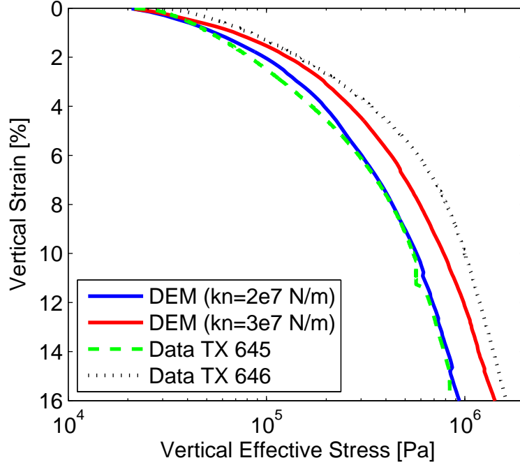
Figure 3-2: Experimental stress–strain curves for sediments from Hydrate Ridge [93], and comparison with DEM simulations for two different values of the grain stiffness.
