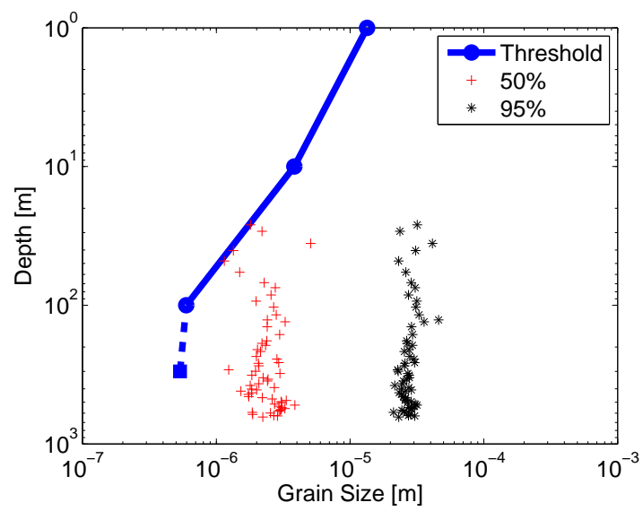
Figure 3-17: Grain-size distribution from site 994 of Blake Ridge [27] overlaid on plot of threshold grain size between capillary invasion and fracture opening as a function of depth.
