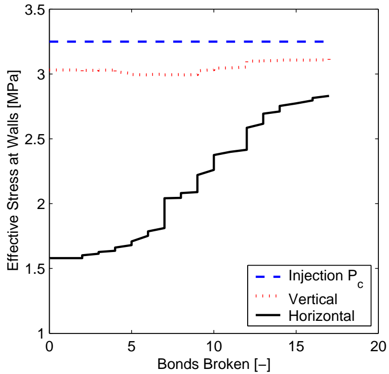
Figure 3-10: Evolution of the vertical and horizontal mean effective stress during fracture propagation for the simulation shown in Figure 3-9. The invading gas pressure remains constant throughout, but the vertical and, especially, the horizontal stress at the boundaries increase during fracture growth. The boundaries introduce an artificial stiffness in the problem that results in an overestimation of the gas invasion pressure.
