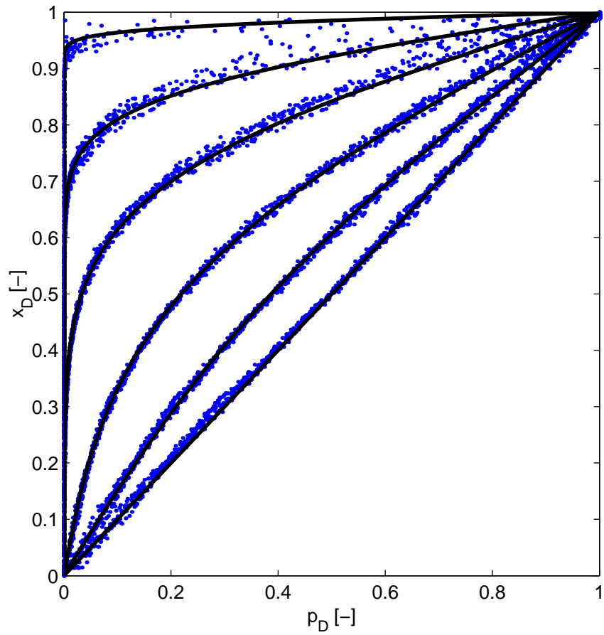
Figure 3-5: Evolution of pressure profiles during the uniaxial fluid flow test. Comparison of DEM simulation (dots) and analytical solution (solid line) at different dimensionless times: \tau = 0.000242, 0.00671, 0.0275, 0.0829, 0.175, 1.404 .
