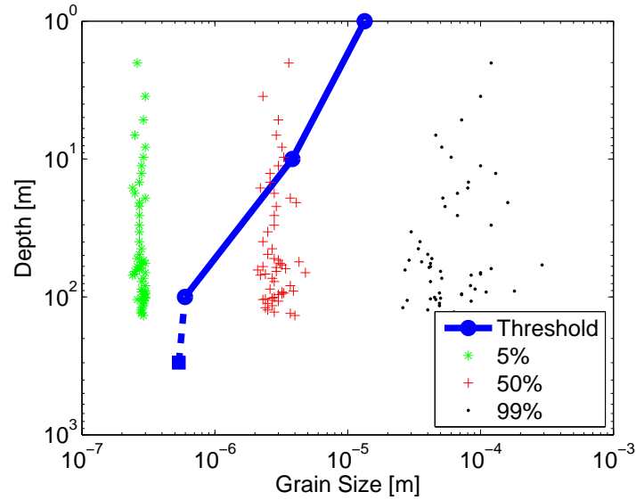
Figure 3-16: Grain-size distribution from site 1246b of southern Hydrate Ridge [30] overlaid on plot of threshold grain size between capillary invasion and fracture opening as a function of depth.
