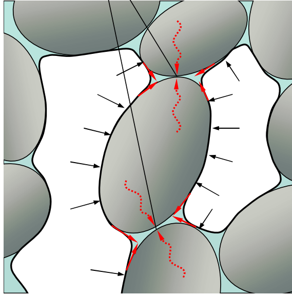
Figure 2-10: Meniscus pinning in the presence of two fluid phases in the sediment. During multiphase flow in porous media, the least wetting phase (gas, white) migrates through the center of the pores, while the most wetting phase (brine, blue) coats the grains (gray) and forms filaments around the crevices of the pore space. This configuration leads to gas–water menisci around the grain contacts. Due to interfacial tension (solid red arrows), these menisci are responsible for an attraction force between grains (dotted red arrows). At the macroscopic level, this can be interpreted as an increment in the cohesion of the material. This is a purely multiphase-flow effect, not present in single-phase poromechanics.
