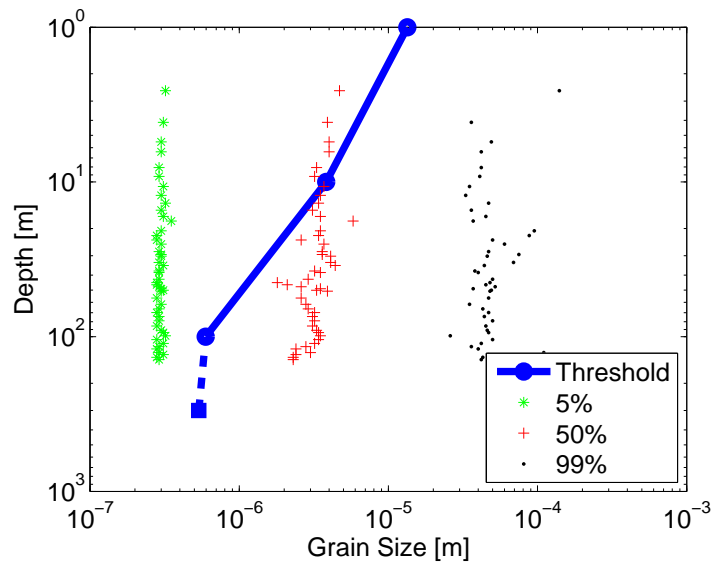
Figure 3-14: Grain-size distribution from site 1244e of southern Hydrate Ridge [30] overlaid on plot of threshold grain size between capillary invasion and fracture opening as a function of depth.
