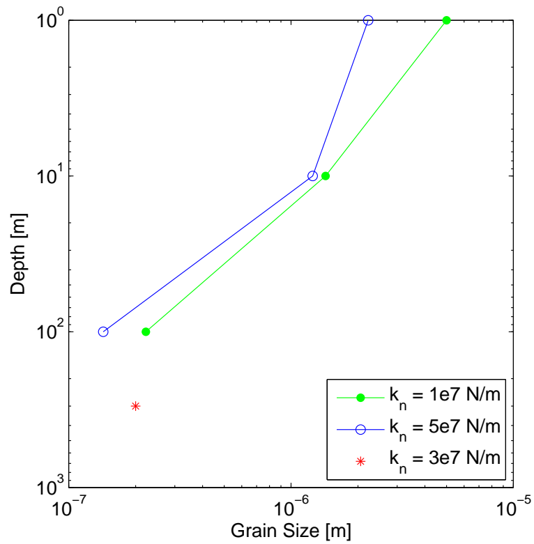
Figure 3-12: Plot of threshold grain diameter between capillary invasion and fracture opening as a function of depth and grain contact stiffness during gas invasion simulations. In sediments with grain sizes smaller than the fracturing threshold, gas invasion occurs by fracture opening. DEM packings with stiffnesses of 1 \times 10^7 N m -1 and 5 \times 10^7 N m -1 exhibit stress-strain behavior that bounds the softest and stiffest curves, respectively, of stress-strain curves of southern Hydrate Ridge. The stiffness of 3 \times 10^7 N m -1 gives intermediate behavior.
