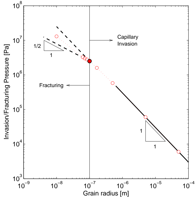
Figure 3-11: Plot of invasion pressure vs. grain size (red circles) for a sediment under 3MPa vertical effective stress (sediment column depth of about 300m). The red-filled circle denotes the critical grain size at which the transition in the mode of gas invasion occurs. For larger grain size, gas invades by capillarity. For smaller grain size, it invades by opening a fracture. In the capillarity-dominated regime, the invasion capillary pressure decreases with increasing grain size with a slope of -1 (black solid line), consistent with the theory (Equation (3.10)). In the fracture-dominated regime, the invasion capillary pressure increases with decreasing grain size, though the predictions of linear elastic fracture mechanics (black dashed line with slope -1/2 ) are not in agreement with our coupled grain-scale model. This suggests the effects of capillarity and inelastic material behavior cannot be neglected.
