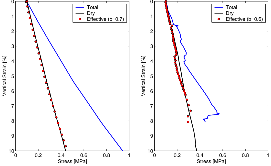
Figure 3-6: Stress–strain curves for uniaxial undrained compaction. The total stress in the fluid-filled sample (blue solid line) is higher than the stress in the “dry” sample (black solid line). The effective stress curve (red circles) is obtained by subtracting the pore pressure (not plotted) premultiplied by the Biot coefficient from the total stress. An appropriate value of the Biot coefficient is found by matching the effective stress curve with the “dry” stress curve. Left: cemented/cohesive sample. Right: unconsolidated/cohesionless sample.
