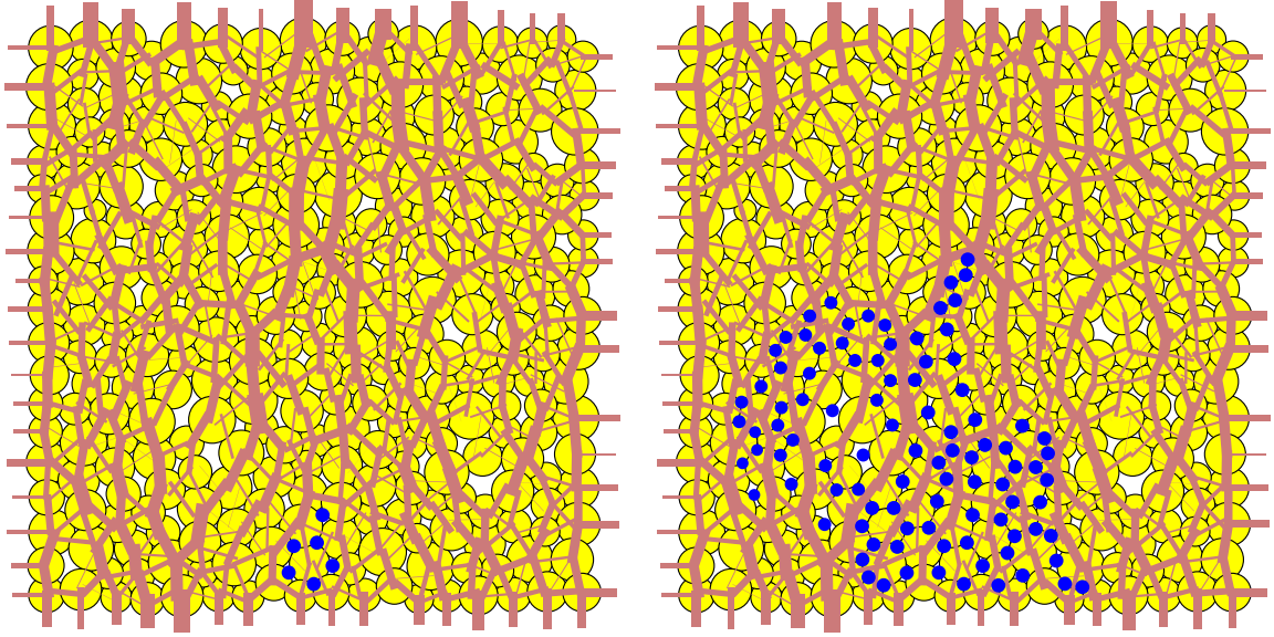
Figure 3-8: Snapshots of the evolution of the methane gas-water interface for the case r_{min} = 50\mu\text{m} . The pores occupied fully by gas are represented with blue dots at the pore centers. The maroon lines indicate compression at grain-grain contacts. The green lines represent tension, which is supported by cohesion between grains. Left: P_c = 5 kPa. Right: P_c = 6 kPa.
