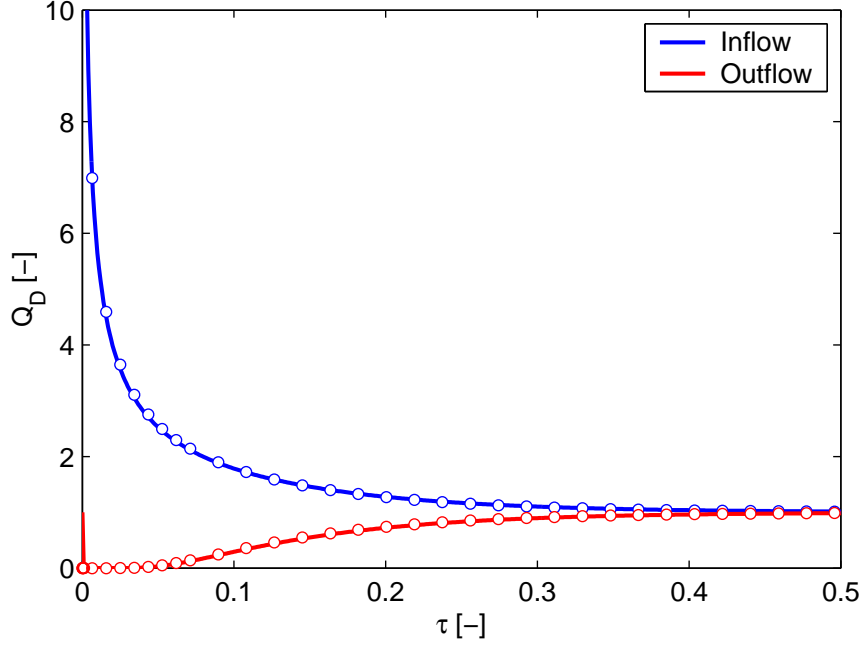
Figure 3-4: Inflow and outflow rates into the pressure cell. Comparison of DEM simulation (circles) and analytical solution (solid line).
