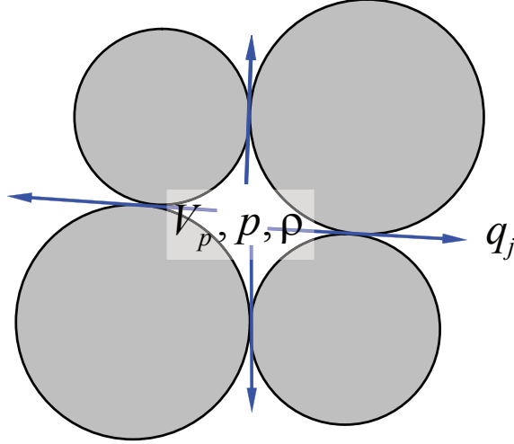
Figure 2-4: Schematic representation of a fluid domain. At any given time, each fluid domain is characterized by its pore volume V_p , and the pressure p and density \rho of the fluid. Fluid can go in and out of the pore domain at a rate q_j into the neighboring fluid domains.
