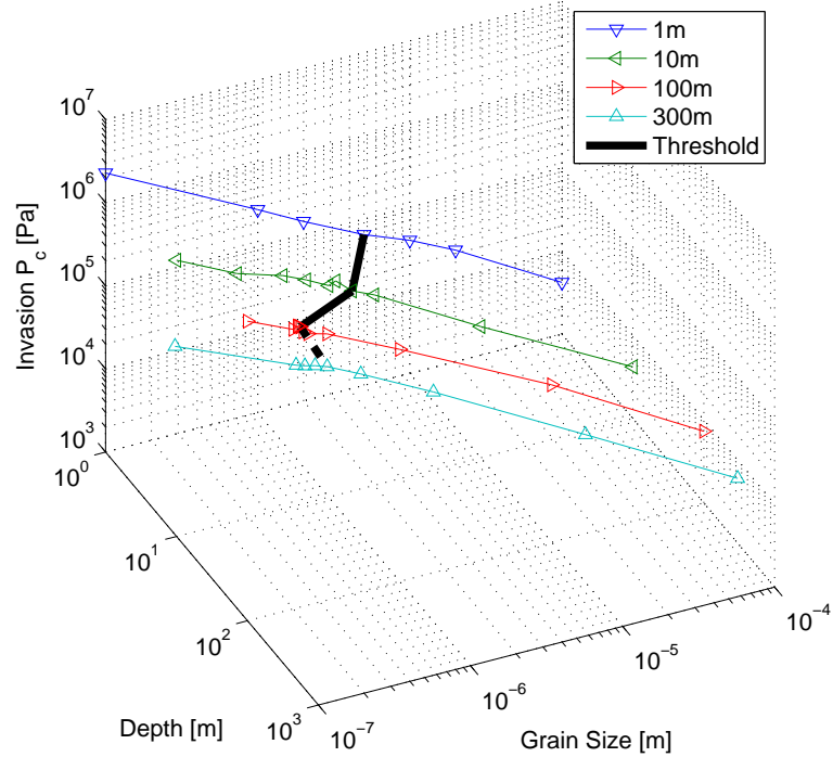
Figure 3-13: Capillary pressure required for gas invasion in soft sediments as a function of depth below seafloor and grain-size. The 300m depth data correspond to slightly stiffer grains. At each depth, for coarser grains than the fracturing threshold value, the slope of the invasion pressure vs grain size is -1 , consistent with the theory (Equation (3.10)).
