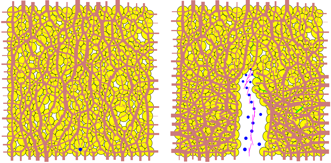
Figure 3-9: Snapshots of the evolution of the methane gas-water interface for an assembly with r_{min} = 0.06 \mu\text{m} . The pores occupied fully by gas are represented with blue dots at the pore centers. The maroon lines indicate compression at grain-grain contacts. The green lines represent tension, which is supported by cohesion between grains. The pink lines show where cohesive bonds were broken. Left: P_c = 3.0 \text{ MPa} . Right: P_c = 3.25 \text{ MPa} .
