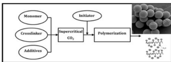
Figure 1. Schematic illustration of synthesis of nano-particle gels in supercritical CO 2 .
