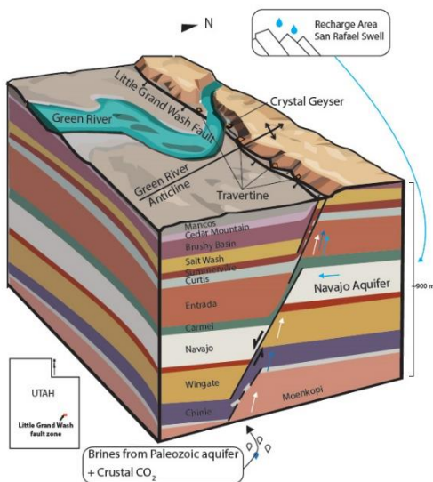
Figure 1: Fractures and faulting noted in potential CO 2 confining layers at the Crystal Geyser site.
