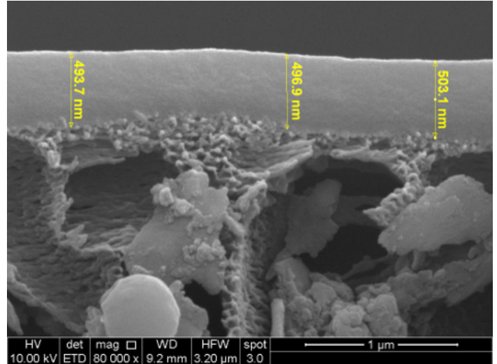
SEM image of an NETL membrane with selective layer coating on a porous support.
