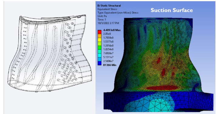
Figure 3. Preliminary cooled turbine blade design with internal cooling features (left) and corresponding stress contours (right) developed by Southwest Research Institute and Purdue University (DE-FE0031929) for a 300 MWe oxy-combustion turbine.
