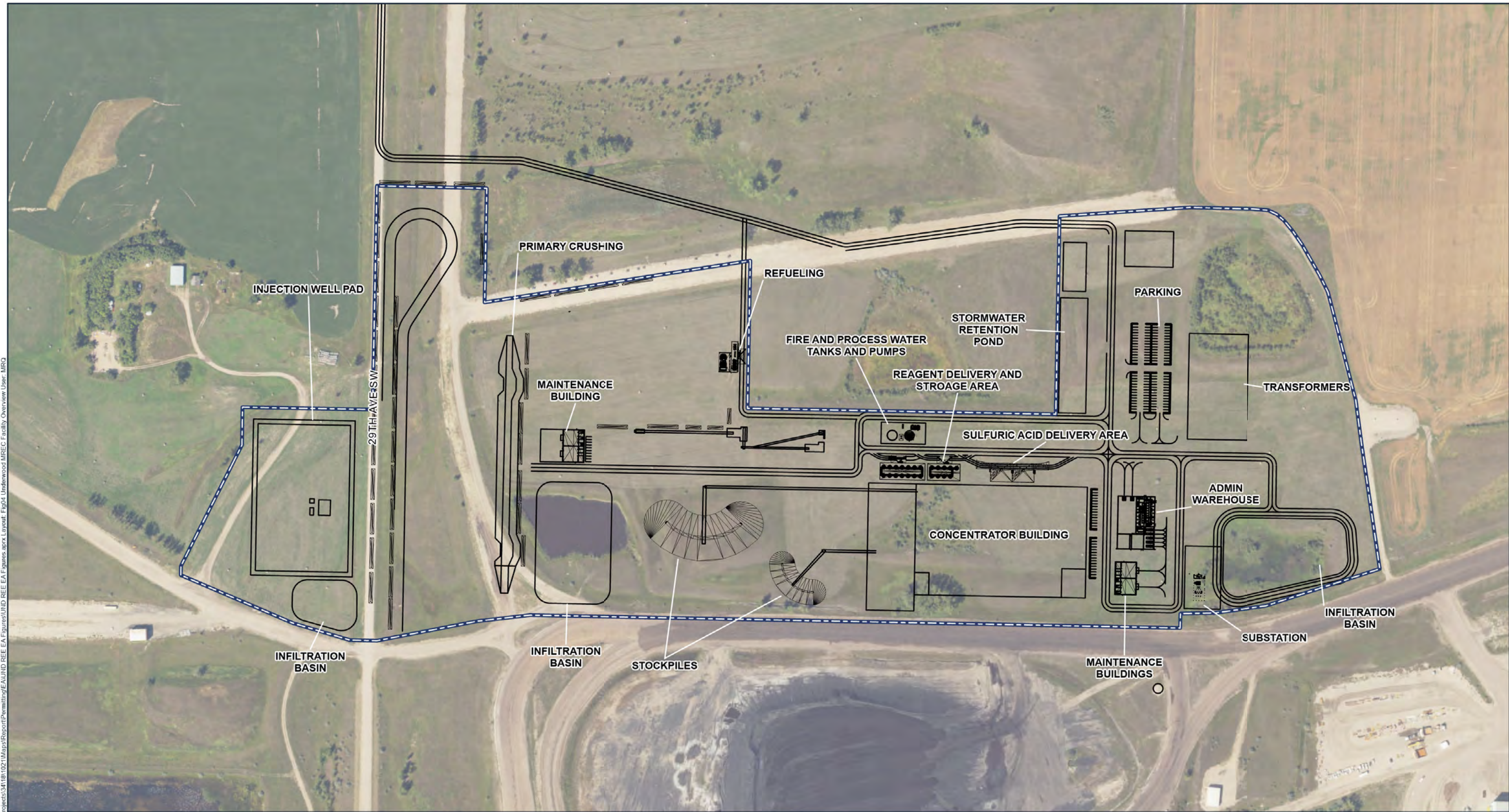
Underwood MREC Facility Overview University of North Dakota Rare Earth Element Demonstration Facilities McLean County, North Dakota FIGURE 4
