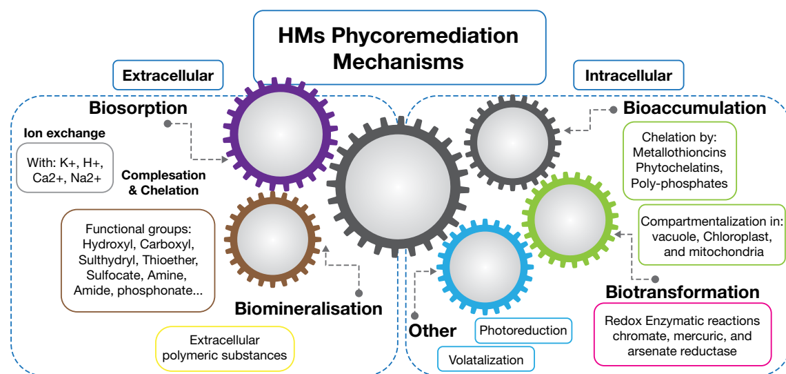
Mechanisms for phytoremediation of heavy metals.
