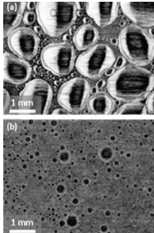
Condensation on (a) uncoated and (b) coated surface with Nelumbo coating.
