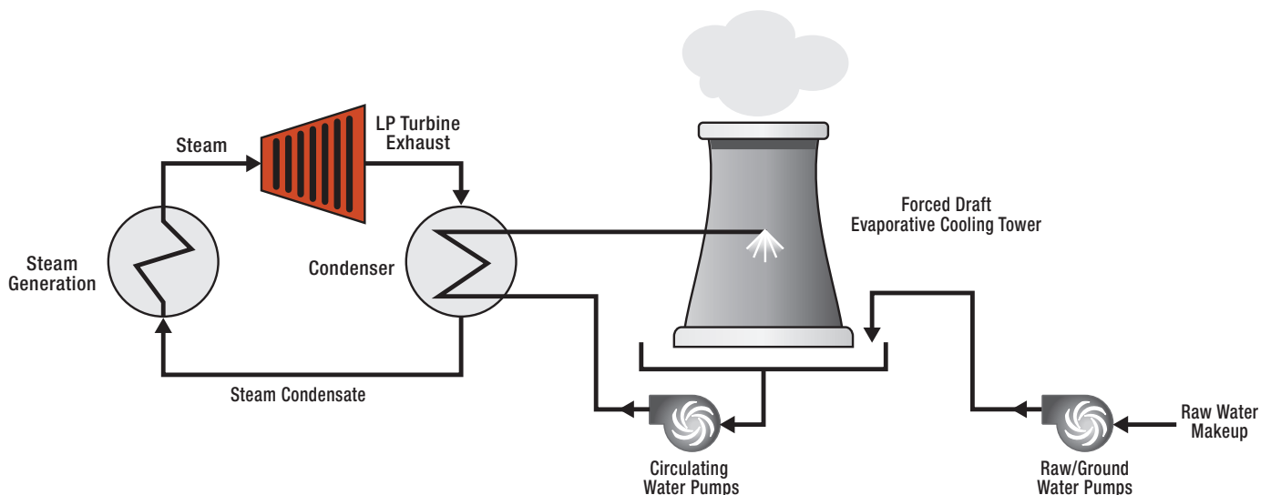
Flow of water in a power plant.
