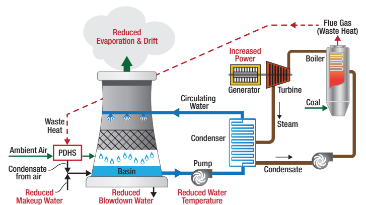
Implementation of sub-dew point cooling tower technology in a coal-fired plant: pressure dehumidifying system (PDHS).
