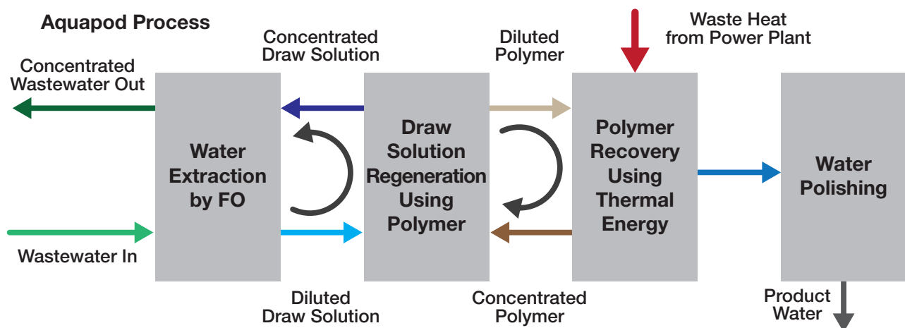
The process utilized by the University of Illinois.
