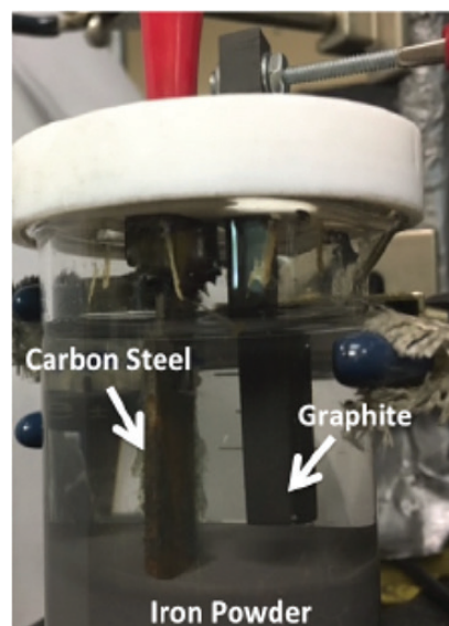
A lab-scale setup for electro-coagulation studies.
