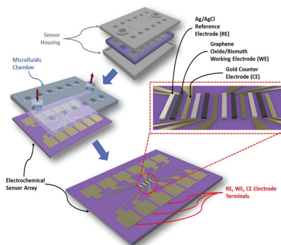
Schematic of electrochemical sensor arrays microanalyzer system.
