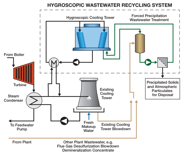
High-level schematic system applied at a full-scale thermoelectric power plant.
