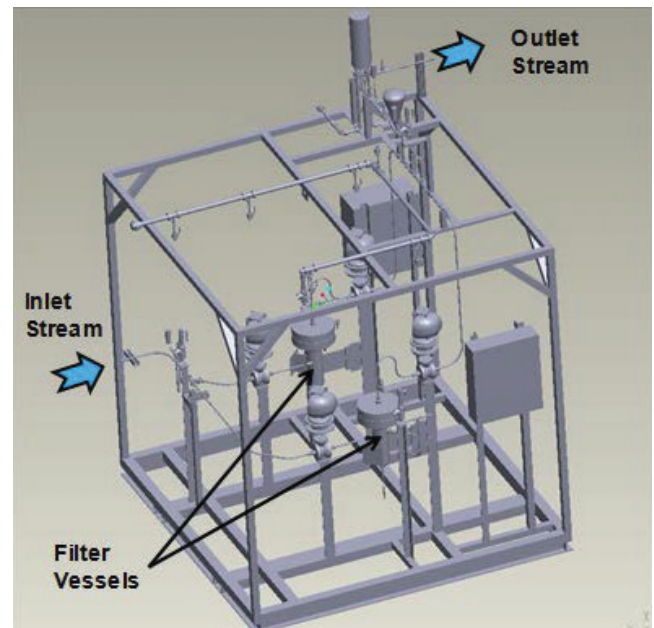
Subscale (1/4 MWth) surface steam generator (produced water testing) skid.
