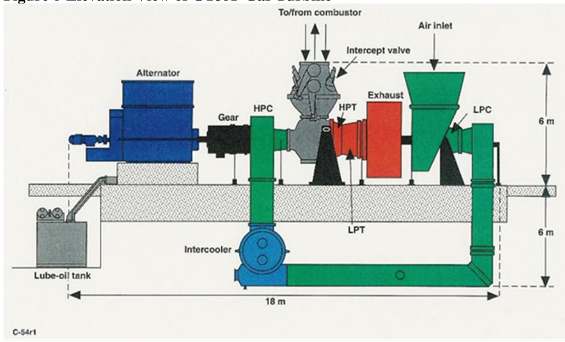
Figure 6- Elevation View of GT35P Gas Turbine
