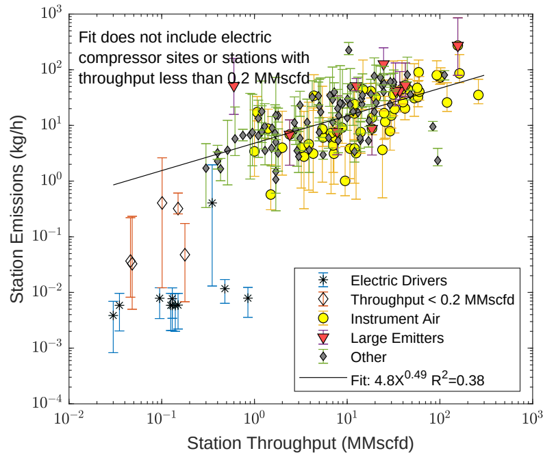
Figure 14: Emission rate as a function of throughput for the 157 stations in the field campaign where throughput data was available. Key characteristics of each station are indicated by point shape, including stations with all electric compressor drivers, stations where gas pneumatics and associated actuators are powered by instrument air, and stations with large emitters. Fit does not include 5 stations with throughput below 0.2 MMscfd or 11 small, all-electric, stations.
