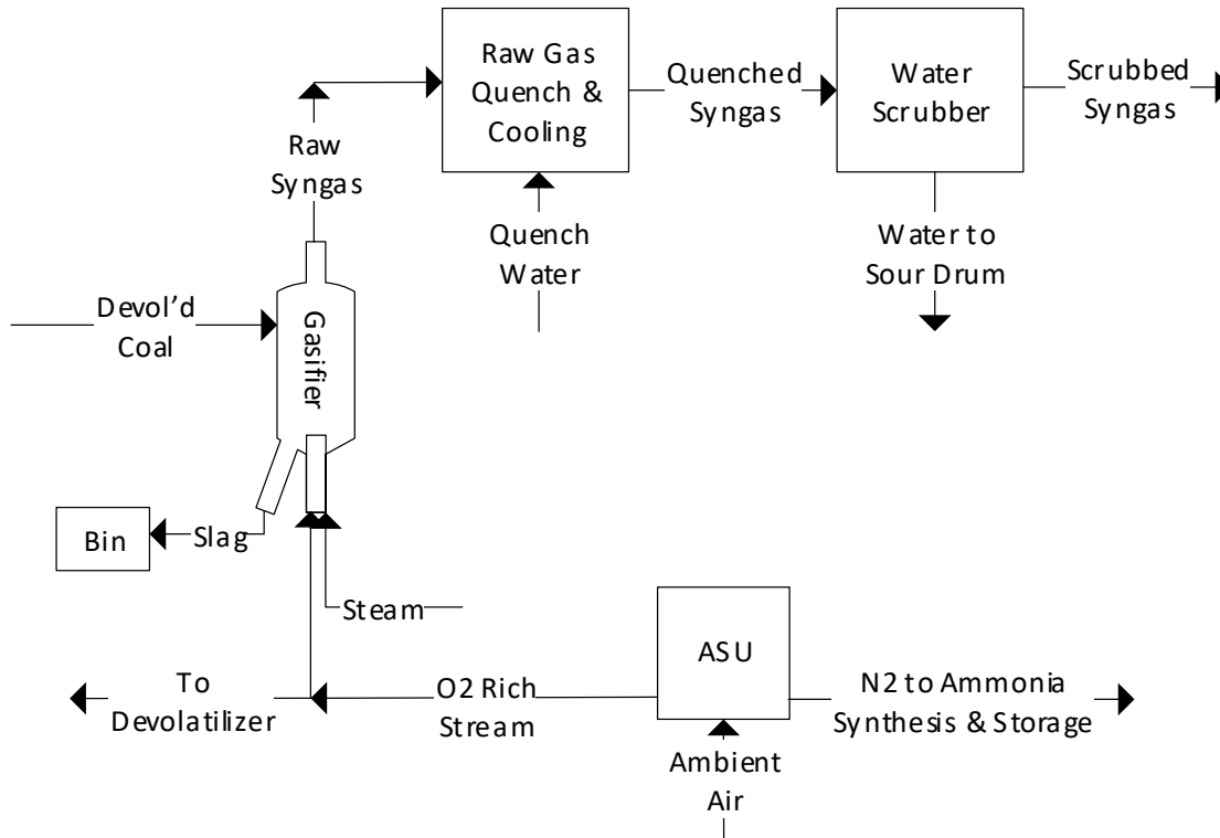
Exhibit A-4 Relevant Stream Composition for ASU, Gasifier, and Quench
