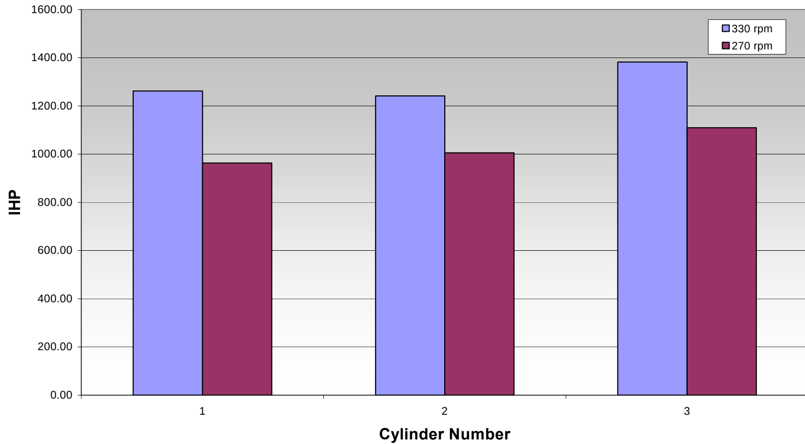
Cylinder IHP
