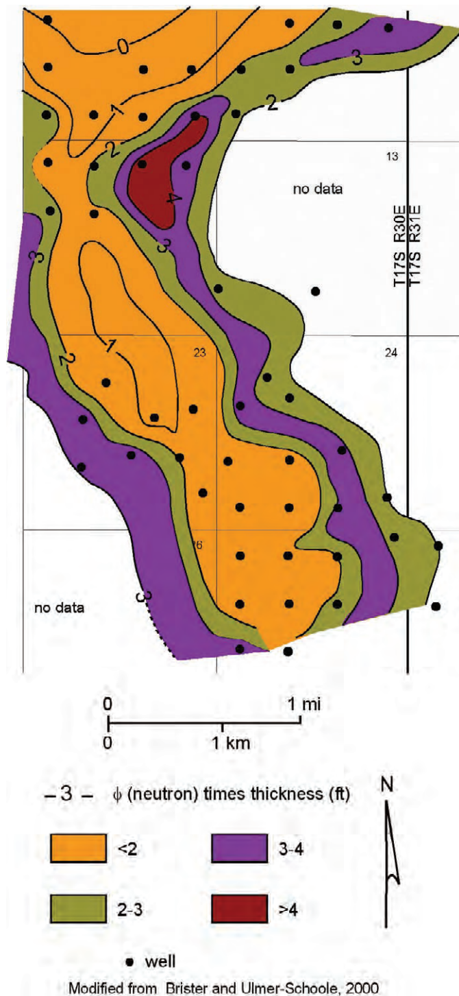
Figure 22. Neutron-porosity-thickness map of Seven Rivers dolograinstone interval, Grayburg-Jackson (formerly Fren) pool, Eddy County. Feature is interpreted to record a tidal-channel deposit. Modified from Brister and Ulmer-Scholle, 2000.
