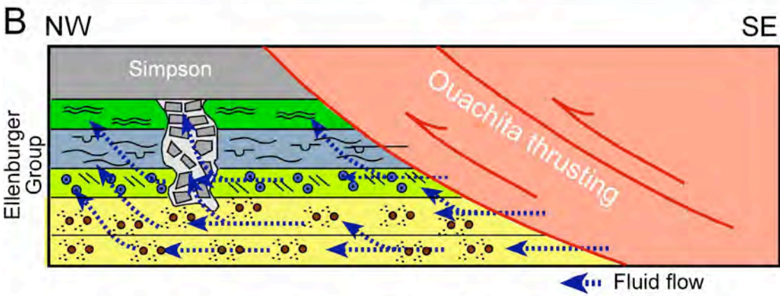
Figure 15. Fluid-flow model of Kupecz and Land (1991) for late-stage replacement Dolomite-L2. Figures from Kupecz and Land (1991). (A) Contour map of \delta O^{18} isotopes of the late-stage replacement Dolomite-L2. Hypothetical fluid pathway-flow lines added by present author. The map indicates that hydrothermal fluids moved from the Ouachita Orogeny front in the southeast toward New Mexico to the northwest. (B) Schematic diagram showing the pathways for the hydrothermal fluids expelled by thrusting during the Ouachita Orogeny. The fluids moved along permeable faults, fractures, karst-breccia zones, and matrix pore-rich units.
