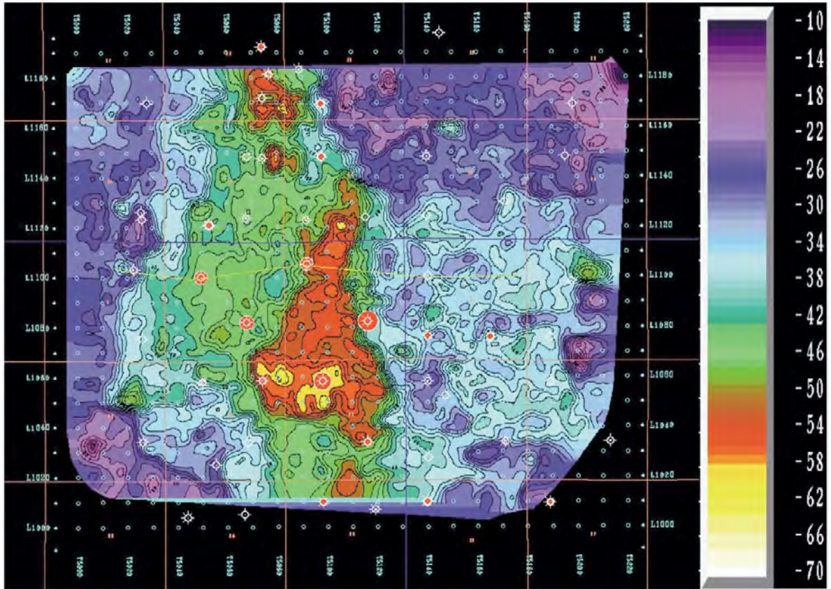
Figure 33. Atoka Formation (top) to Chester (base) isochron map illustrating valley-fill-type geometry (red) of sands in Buffalo Valley field. Modified from Van Dok and Gaiser (2001).
