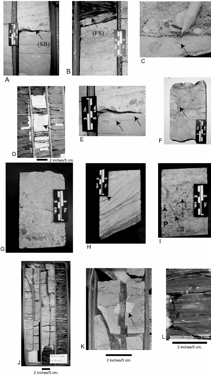
Figure 16. Key features identifiable in core (A) basal Morrow sequence boundary, (B) flooding surface at top of fluvial succession, (C) basal bayfill delta disconformity ( Glossifungites surface), (D) transgressive lag at major flooding surface, (E) sand-filled burrows at base fluvial unconformity ( Glossifungites surface), (F) pedogenic fractures in the Mississippian Chester Formation, (G) medium to coarse pebbly arkosic sand, (H) potential tidal influence (reactivation surface and double mud drapes), (I) bioturbated zone (includes Skolithus , Planolites , and Teichicnus ), (J) laminated central “basin” estuary shale overlain by distal bayhead delta facies, (K) solitary coral from upper bayhead delta facies, and (L) marine shale above major flooding surface (modified from Bowen and Weimer, 2004). Note that all photos are related to core description and facies shown in figure 17.
