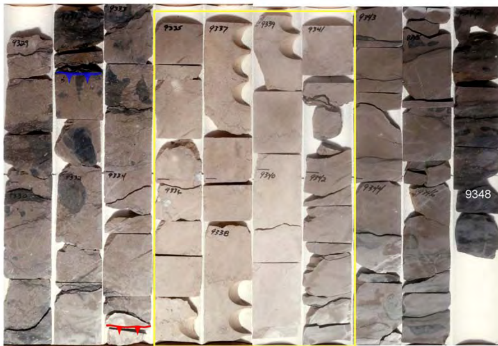
Figure 35. Core photograph, description, wireline-log signature, core analysis data, and stable isotope analysis of the Missourian (lower Canyon) interval. Proposed exposure surfaces indicated by red horizontal lines with downward-pointing triangles. Blue vertical bar indicates interval illustrated in core photograph. High-porosity and -permeability reservoir interval outlined in yellow.
