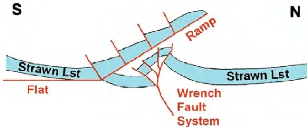
Figure 40. Structural interpretation of Strawn thrust reservoirs in Val Verde Basin. After Khan and others (2002). Model interprets that Strawn interval comprises single overthrust ramp, divided by back thrusts overlying wrench faulted pop-up structures. Model contrasts with those presented by Montgomery (1996) and Newell and others (2003) (figs. 37 and 38).
