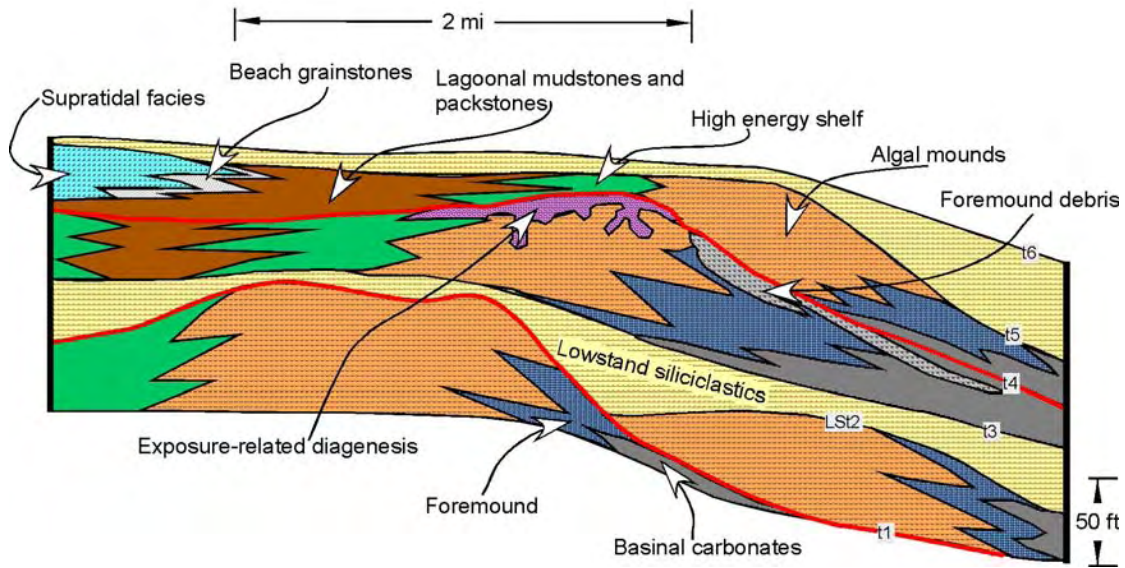
Figure 39. Generalized distribution and architecture of Missourian–Virgilian carbonate succession on the Northwest Shelf (New Mexico) (after Mazzullo, 1998). Red lines on lower schematic indicate sequence boundaries.
