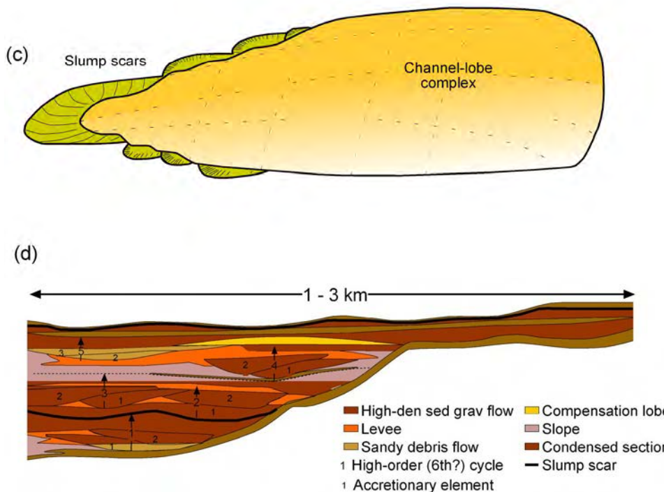
Figure 25. Brushy Canyon depositional cycle models of Gardner (1992): (a) processes during sea-level highstand include restriction of continental siliclastic depositional environments well shelfward of shelf margin, deposition in basin of windblown silt, and gravity transport of shelf-margin carbonate debris; (b) processes during sea-level lowstand include encroachment of prominently eolian depositional environments on shelf margin, accumulation of siliclastics on upper slope, slumping of accumulated siliclastics, and downslope transport of siliclastics by turbidity flow; (c) idealized model of relationship of channel-lobe complex to slump scar; and (d) idealized strike section showing depositional environments, slump scars, and depositional elements of high-order cycles. Slumping may place updip margins of reservoir facies in contact with low-permeability slope siltstones, thus providing updip lateral seal to some reservoirs.
