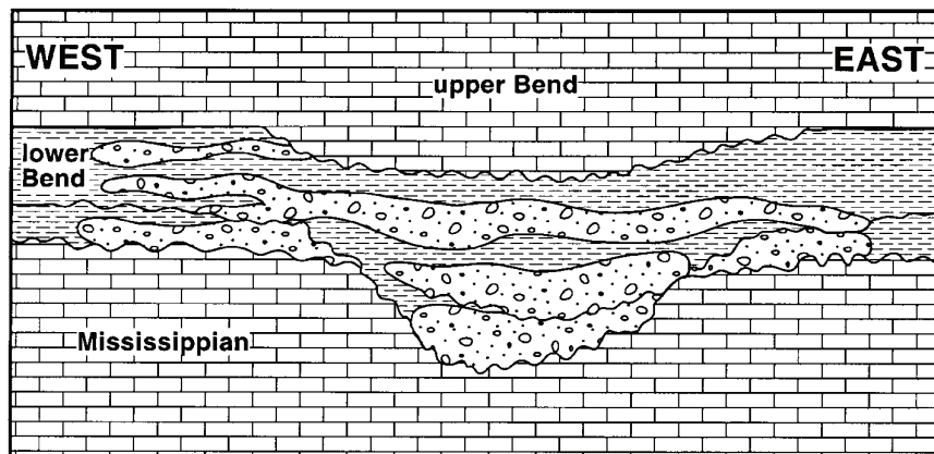
Figure 13. Illustration of incisive and unconfined alluvial channels encased in shale in lower Bend (Atokan age), overlain by dominantly carbonate upper Bend (modified from Brister and others, 2002). Architecture analogous to proximal alluvial facies in Taylor Draw field (Upton County), as well as “lower sand” interval in Vacuum field (Lea County, New Mexico).
