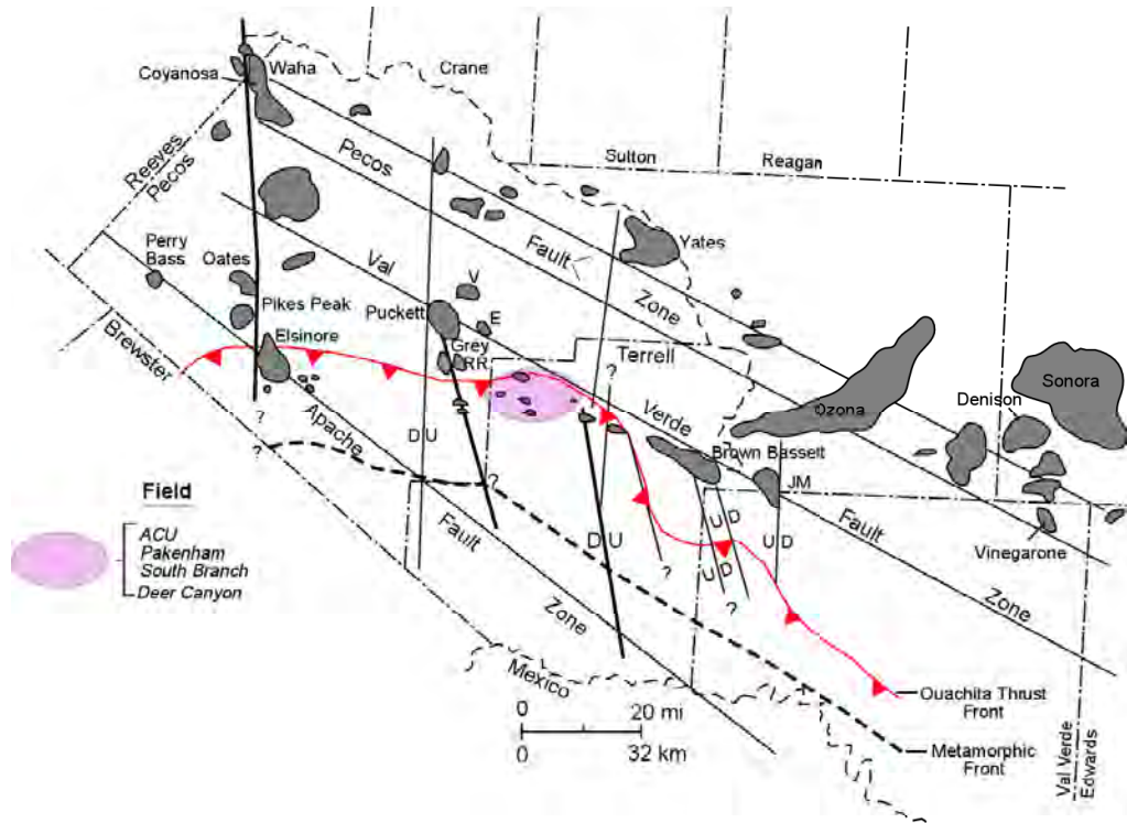
Figure 35. Regional map of the north edge of Val Verde Basin. After Montgomery (1996). Fields highlighted in gray. Most studied region containing Desmoinesian Strawn Formation reservoirs outlined in purple. Region contains ACU, Pakenham, South Branch, and Deer Canyon fields. North edge of Val Verde Basin indicated in red by Ouachita Thrust Front (alternatively called Foreland Thrust).
