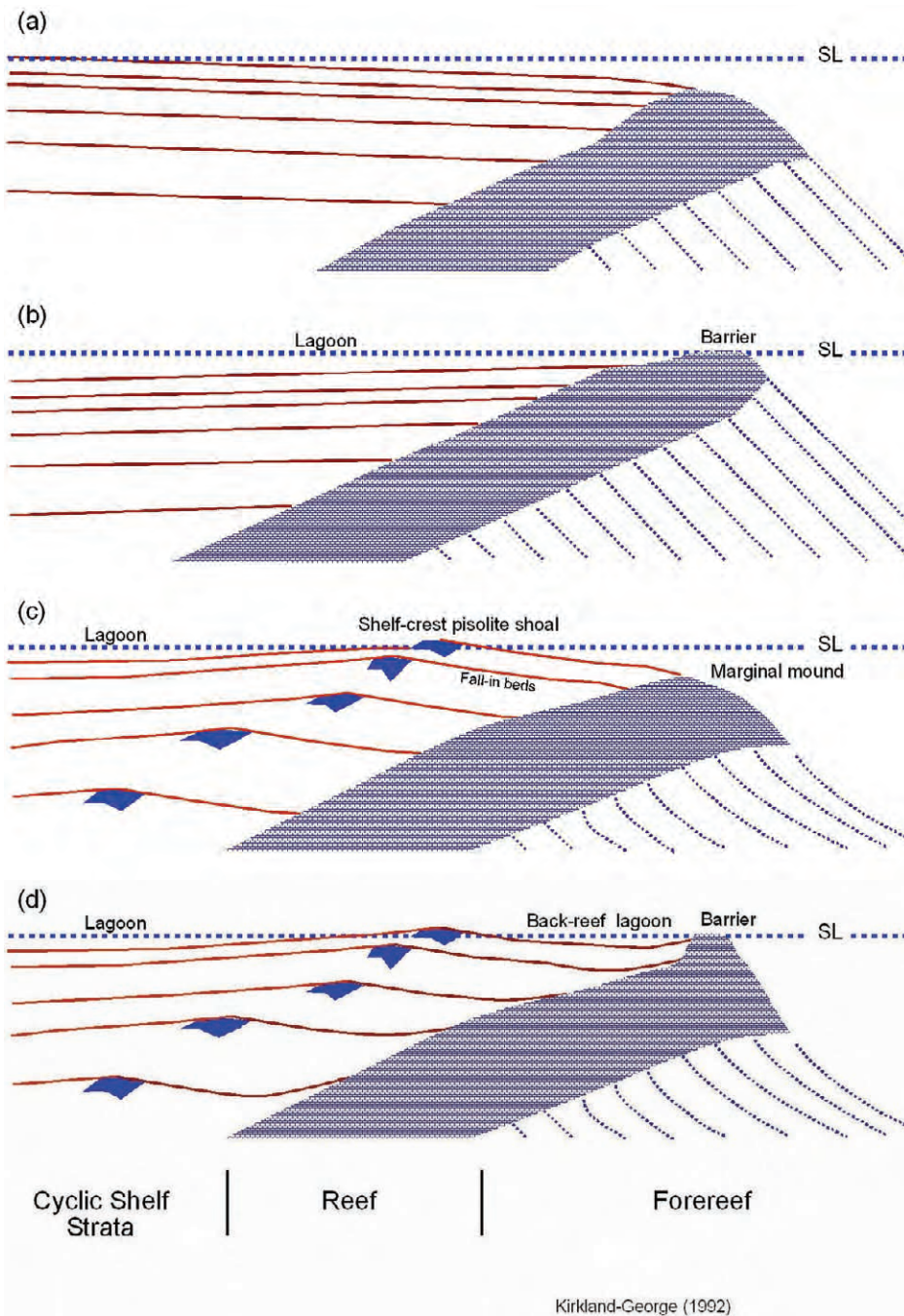
Figure 3. Proposed models for the Guadalupian shelf margin: (a) uninterrupted shelf, (b) barrier reef, (c) marginal mound with pisolite-shoal shelf crest, and (d) barrier island with back-reef lagoon and pisolite shoal. Modified from Kirkland-George (1992).
