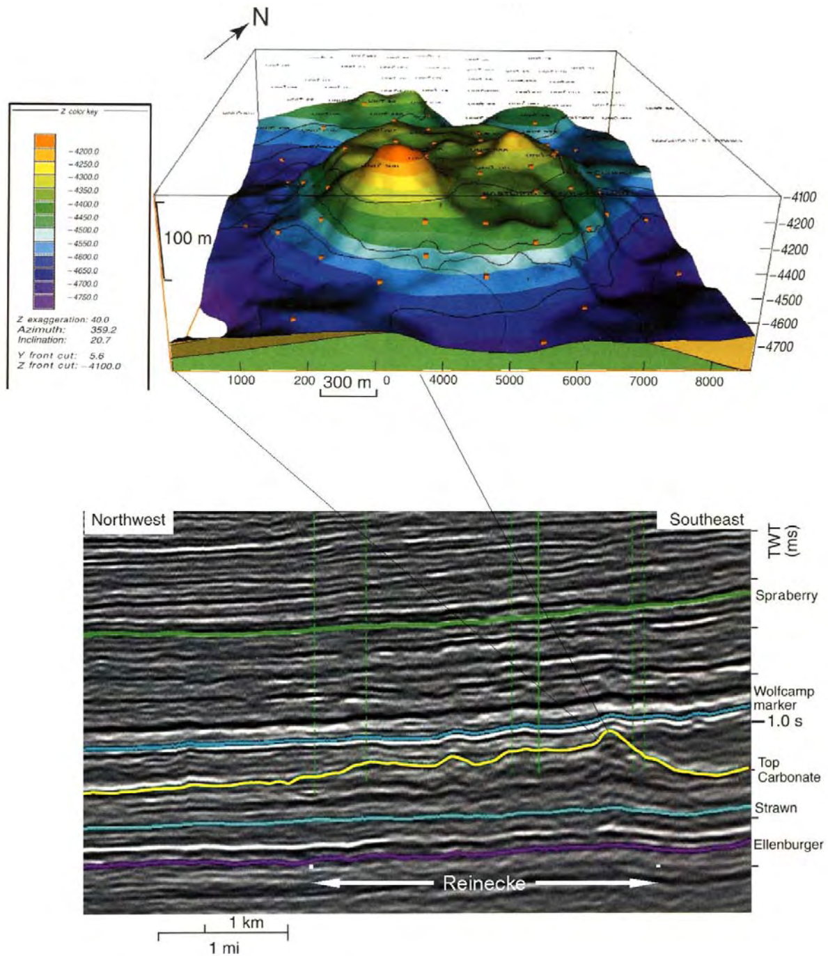
Figure 23. Regional seismic line through Reinecke field (bottom) with inset of the South Dome area, top Virgilian carbonate structural map, based on seismic and well logs. Note that the inset is rotated relative to regional seismic (after Saller and others, 2004). This figure illustrates irregularity of the top Virgilian carbonate surface at both local (<300 m) and regional scale (<3 km).
