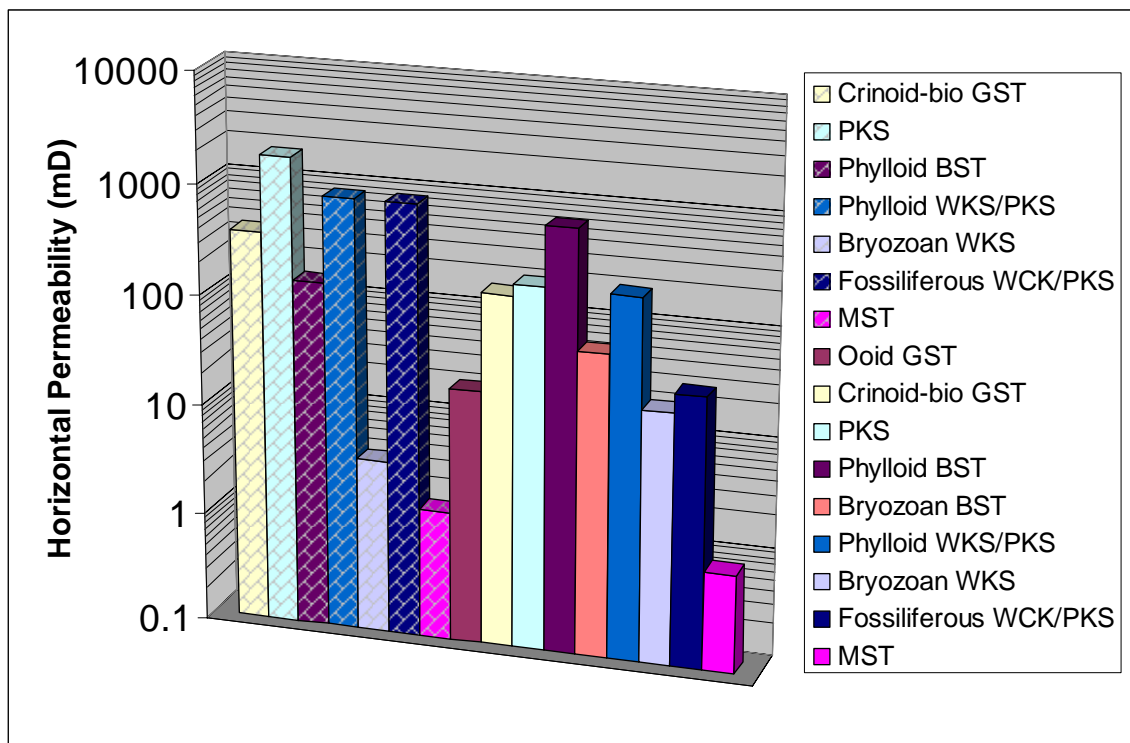
Figure 53. Bar charts comparing porosity and horizontal permeability between undolomitized (no fill pattern) and equivalent, dolomitized (fill pattern) facies at Reinecke field. Data from Saller and others (2004).
