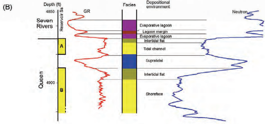
Figure 30. McFarland reservoir: (A) structure map on top of the Queen Formation; State University Units No. 1 and 2 are outlined; and (B) representative well log of the upper Queen productive-sandstone interval. Production is from interpreted tidal-channel and shoreface (probable beach ridge) sandstone. Supratidal carbonate provides baffle between productive sandstones. Modified from Holtz (1994).
