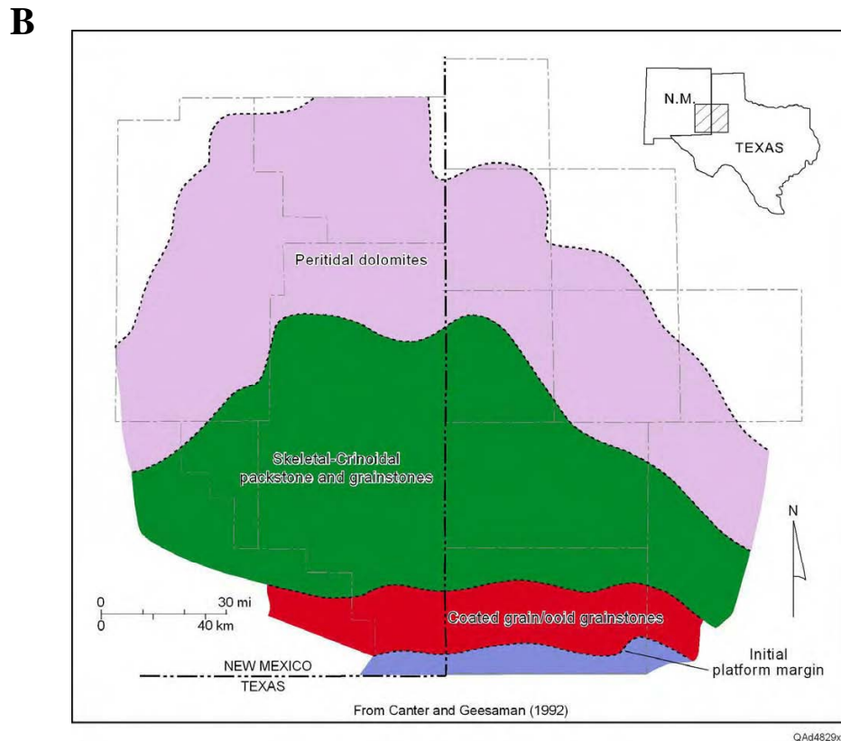
Figure 18. Paleogeographic reconstructions of Wrusten Group depositional environments during the middle Silurian. A. General regional model depicting northern platform and southern, outer platform – basin. Platform rocks comprise Fasken platform-margin buildup successions and inner platform shallow subtidal to tidal-flat sediments. Coeval, argillaceous mudstones of the Frame Formation and underlying Wink Formation were deposited south of the platform margin in a slope/outer platform setting. From Ruppel and Holtz, 1994. B. Reconstruction on northern platform area showing east-west striking facies belts and general northward shallowing of facies tracts. From Canter and others, 1992.
