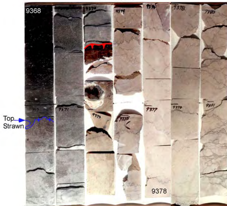
Figure 33. Core photograph, description, wireline-log signature, core analysis data, and stable isotope analysis of the lowermost Missourian (lower Canyon) interval. Proposed exposure surfaces indicated by red horizontal lines with downward-pointing triangles. Note that highest gamma-ray log readings occur above the exposure surface in the overlying crinoidal wackestones of the Missourian succession. Blue vertical bar indicates interval illustrated in core photograph.
