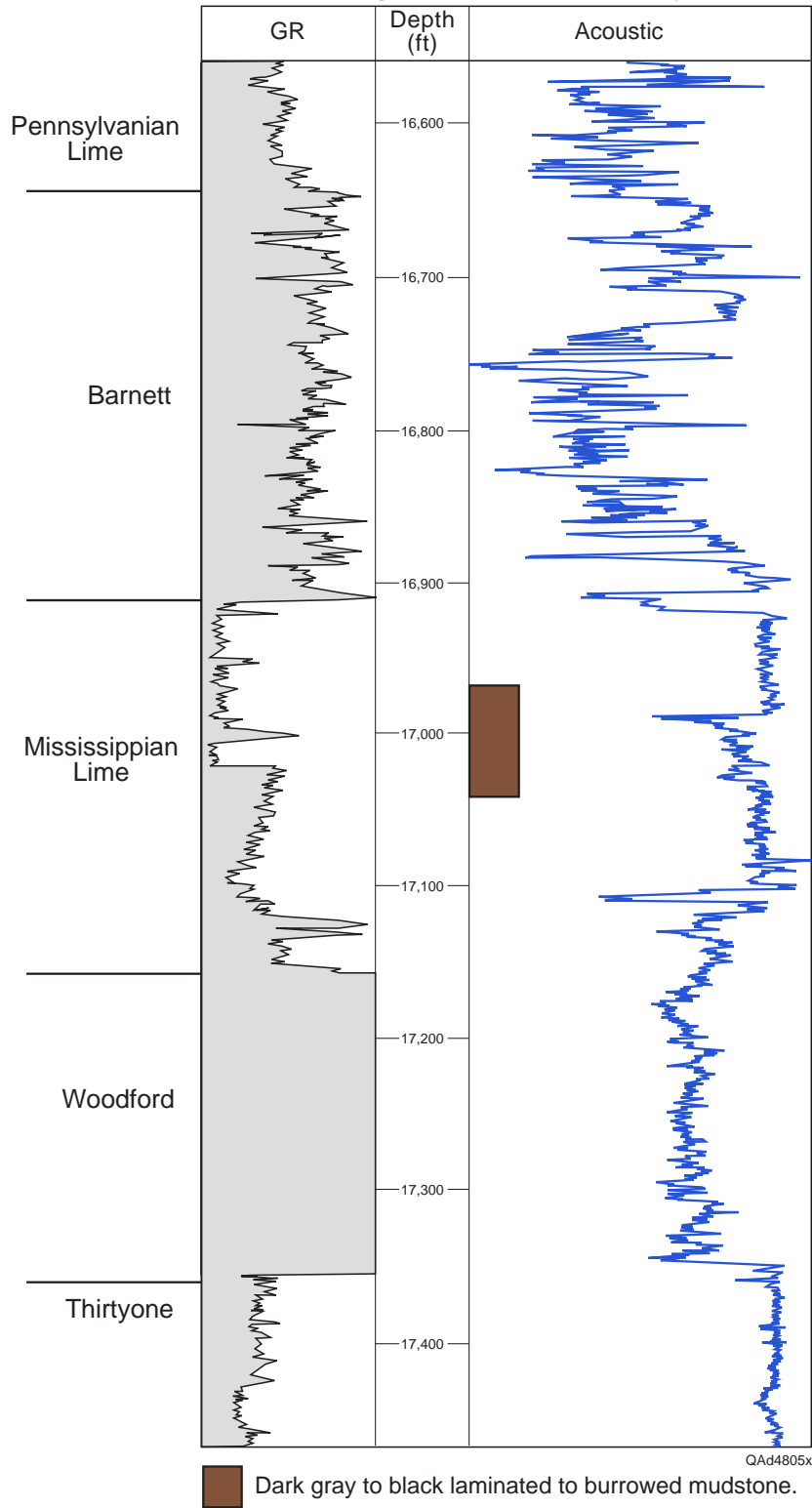
Figure 11. Typical wireline log signature from Mississippian cored well in the southern Permian Basin.
