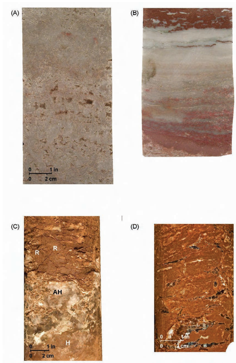
Figure 14. Artesia Group evaporite facies (University No. 3210-2 well, Embar field, Andrews County): (A) Yates Formation brine-pool, vuggy to massive, nodular anhydrite; vugs are filled with halite and may be molds after gypsum crystals; alternatively, vuggy interval may be fenestral tidal-flat carbonate that has been replaced by sulfate; (B) Yates brine-pool, plane-laminated anhydrite may record cycles of gypsum growth and abrasion in a shallow pool; (C) brine-pool and brine-pool-margin (sabkha) succession of mosaic halite, anhydritic halite, and mudrock residue after dissolution of halite from mixed halite-mudrock facies; and (D) sabkha, silty, very fine grained sandstone containing cm-scale halite crystals. Dissolution of halite would produce haloturbated sandstone such as is shown in figure 13D.
