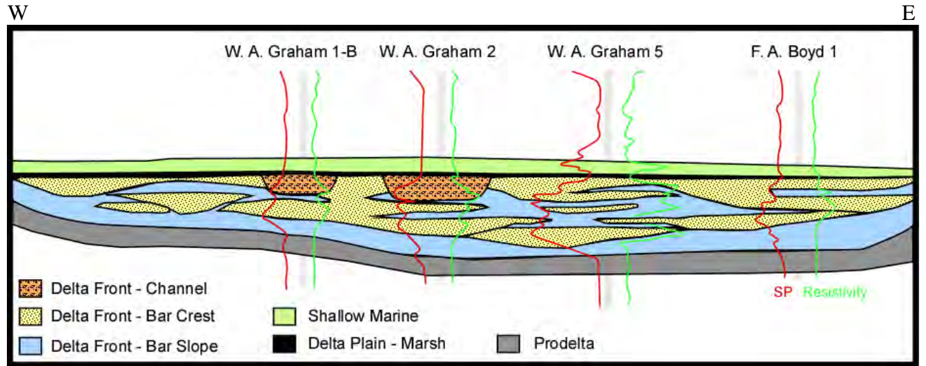
Figure 11. West-east, strike-oriented cross section of the 'Gray Interval,' West Tuscola field, Taylor County (after Shannon and Dahl, 1971). Entire thickness represented by wireline logs approximately 195 ft. The schematic representation of superimposed lowstand channels on a highstand delta in figure 9 may be representative of this field.
