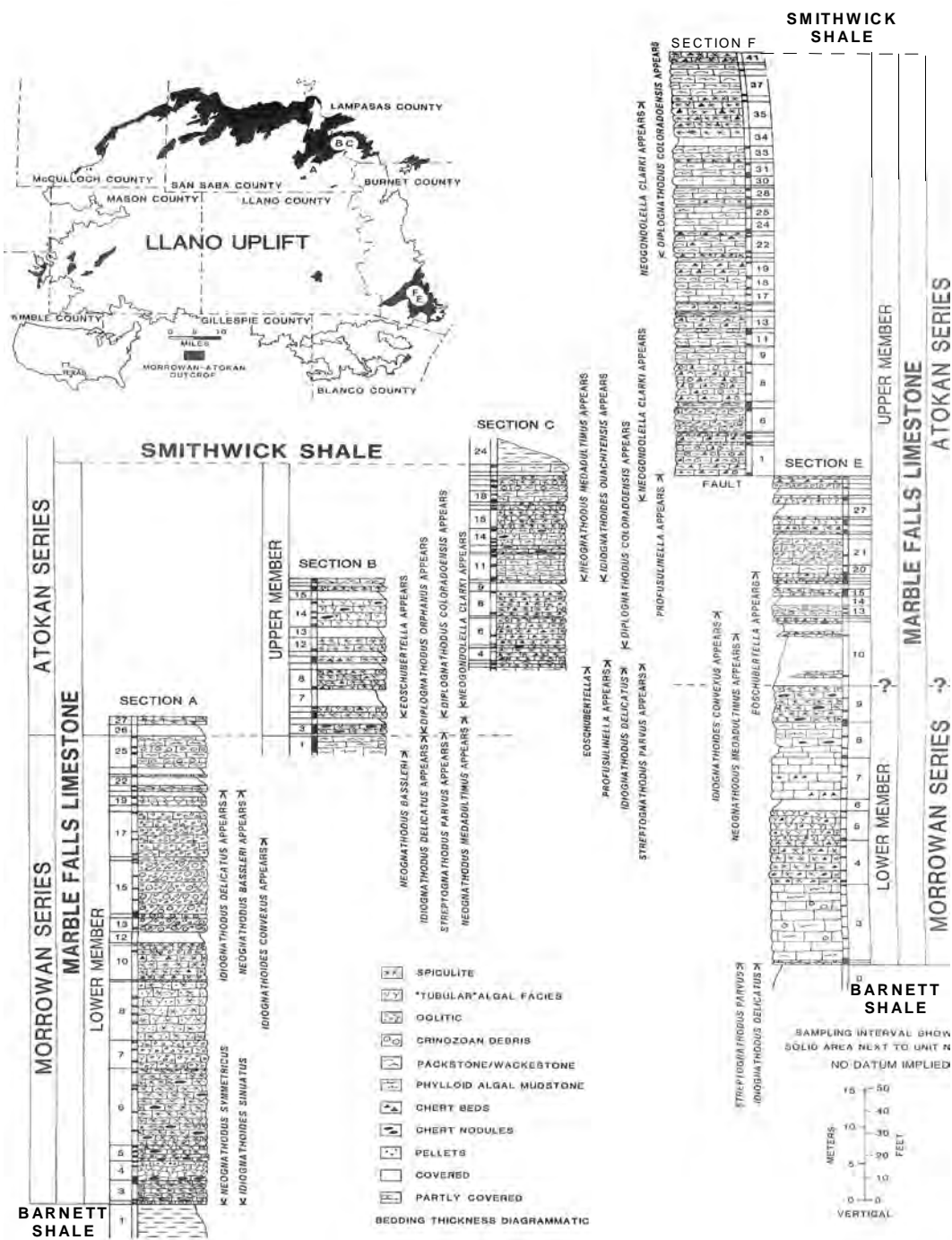
Figure 39. Regional outcrop correlation of Lower and Upper Marble Falls Formation along the east-northeast margin of Llano Uplift (modified from Manger and Sutherland, 1984). Note higher energy facies (oolites dominate) in section A compared with that of section E.
