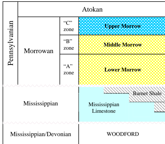
Figure 8. General stratigraphic column for Mississippian- and Pennsylvanian-age units in Northwest Delaware region of the Permian Basin (modified from Coker, 2003). Within Morrowan-age units the yellow fill in the Lower and Middle Morrow indicates a dominance of siliciclastic deposition in that area, whereas the blue fill of the Upper Morrow indicates carbonate deposition.
