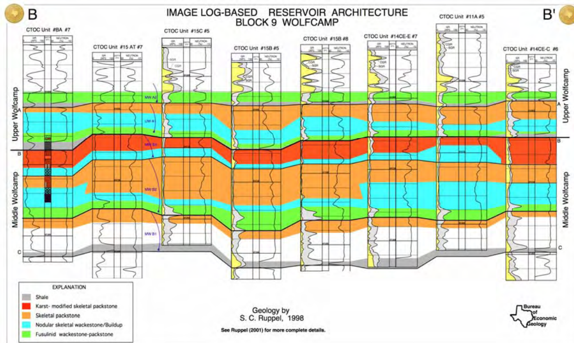
Figure 5. Example of reservoir cross section produced during the project (Wolfcamp, Block 9 field, Andrews County, Texas).
