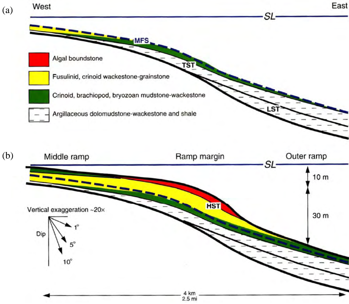
Figure 41. Depositional models for high-frequency stratigraphic architecture of South Dagger Draw field, New Mexico (after Tinker and others, 2004). (a) Facies distribution and depositional environments for lowstand and transgressive systems tracts (LST and TST). Note limited proportion of high-energy facies and their restrictions to the middle ramp area. (b) Facies distribution and depositional environments for highstand systems tract (LST and TST). Note basinward step of HST relative to LST and TST and dominance by higher-energy facies and algal boundstones. Note that water depths even at the ramp crest are thought to be in excess of 10 m.
