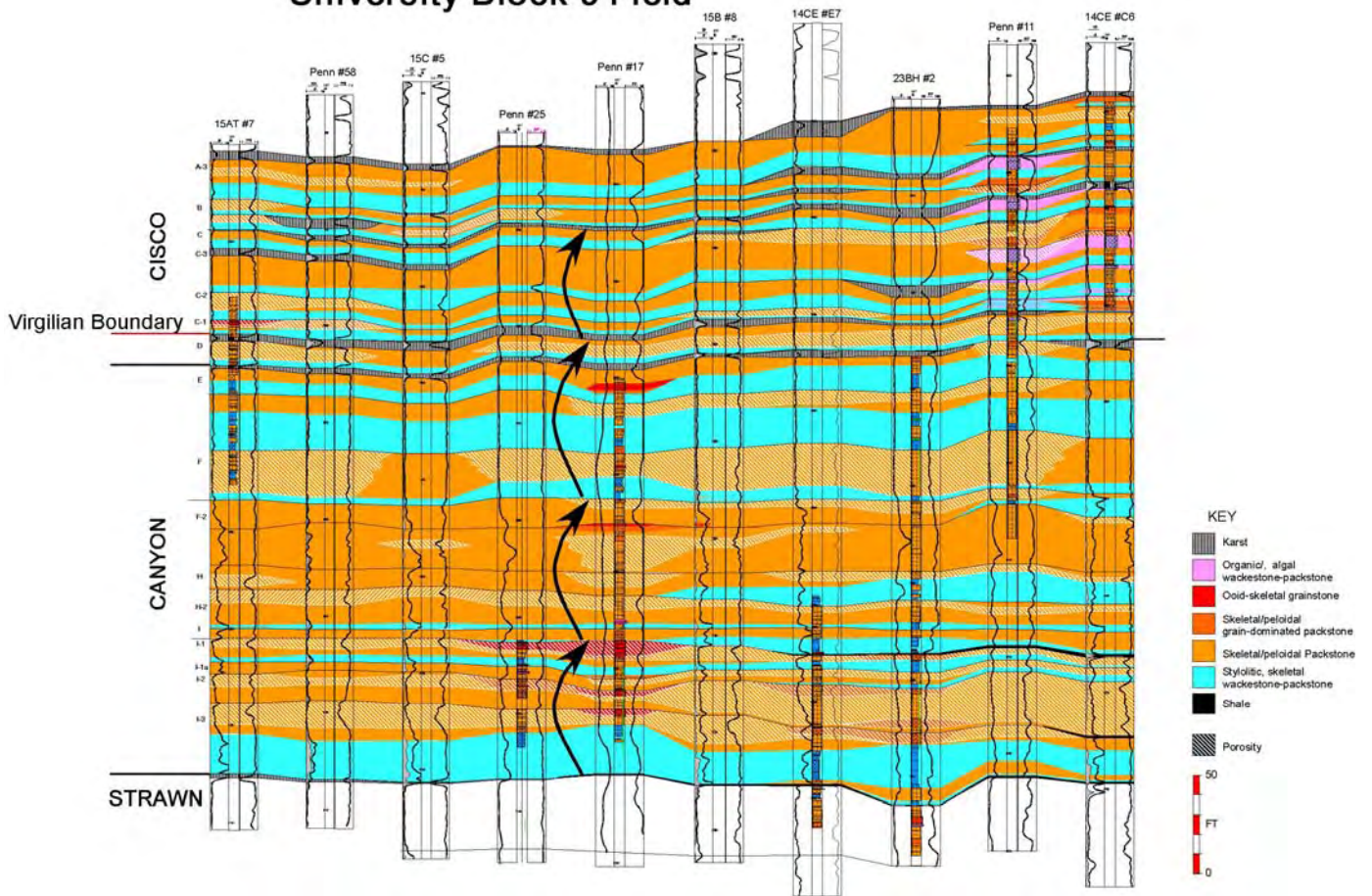
Figure 47. Regional core, FMI, and well-log-based correlation across University Block 9 area (modified from Barnaby, unpublished). Porous zones indicated by inclined hatch marks. The most regionally pervasive high-porosity zone is in cycle F, which is upper Canyon as defined by Saller and others (1999b). Note presence of algal wackestones and packstones in Penn #11 and 14CE #6 wells in the Virgilian succession.
