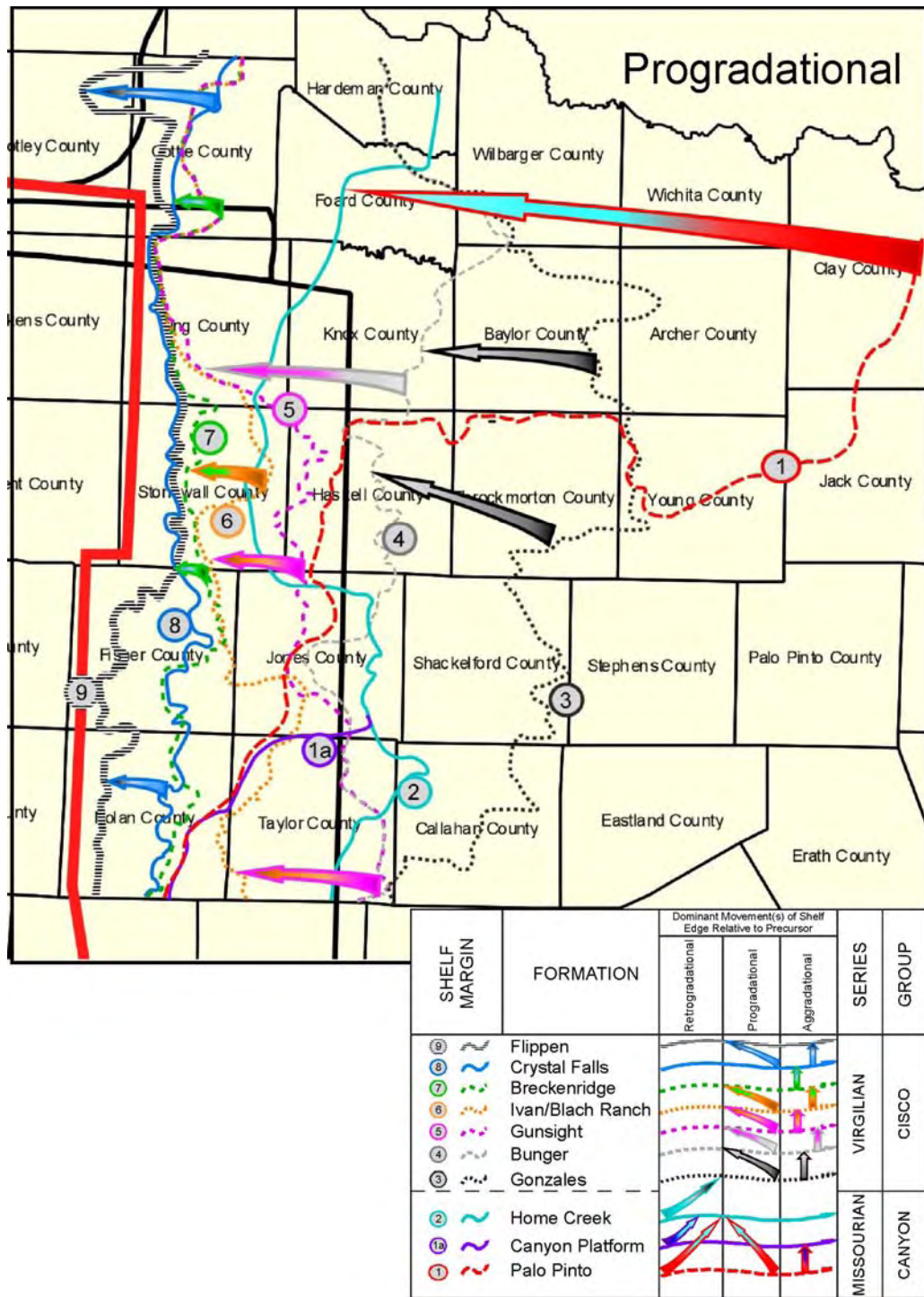
Figure 16. Progradational carbonate shelf margin trends for the Missourian and Virgillian Series (after Brown and others, 1990). Note that shelf margin 9 (Flippen Formation) does not pass into the Permian Basin (as defined by this study). Siliciclastic sediments are trapped largely behind this margin during the Virgillian.
