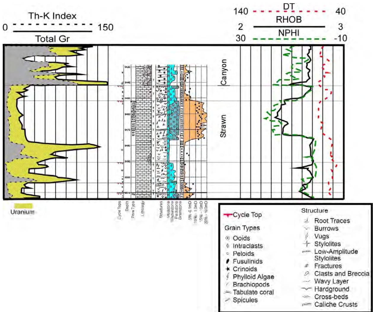
Figure 24. Core description, wireline-log signature, and core-analysis data for a Stage 2 alteration episode. This interval is at the top of the Strawn Formation in Parker X#1 well. Note that there are five cycle tops (each with possible exposure) interpreted by Saller and others, 1999. Exposure event at 9,452 ft 6 inches has no visible manifestation on spectral gamma-ray log. Interval above top of Strawn characterized by high thorium peak, indicating exposure. Total gamma spike at 9,480 ft appears to represent a small flooding or deepening event. In the absence of spectral gamma, exposure surface at 9,440 ft (top of Strawn) would probably be interpreted solely as a flooding event.
