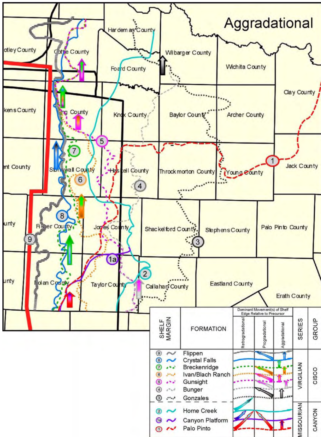
Figure 15. Aggradational carbonate shelf margin trends for the Missourian and Virgillian Series (after Brown and others, 1990). Note that the aggradational component of each trend varies along strike. Color fill of arrows corresponds to color of older margin at the base and new margin location at the arrow tip.
