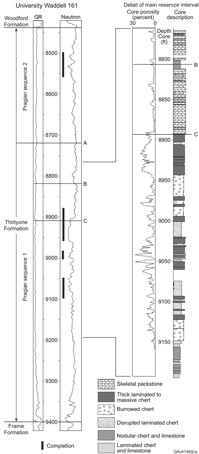
Figure 16. Reservoir facies at University Waddell field. From Ruppel and Barnaby (2001).
