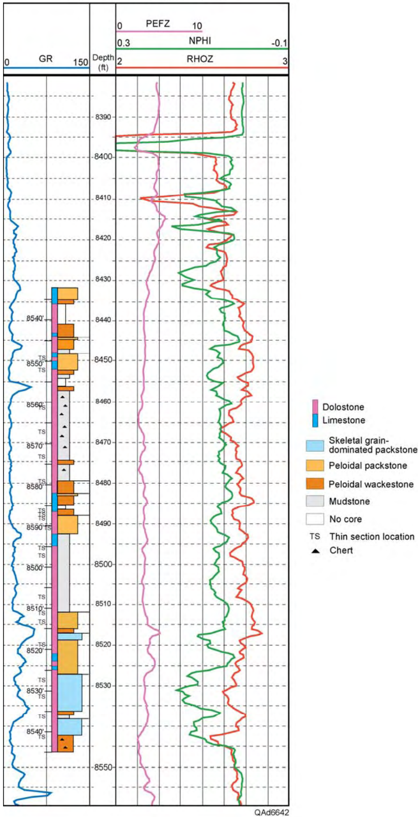
Figure 20. Description of the Montoya cored section in the Dollarhide 25-2-S well.
