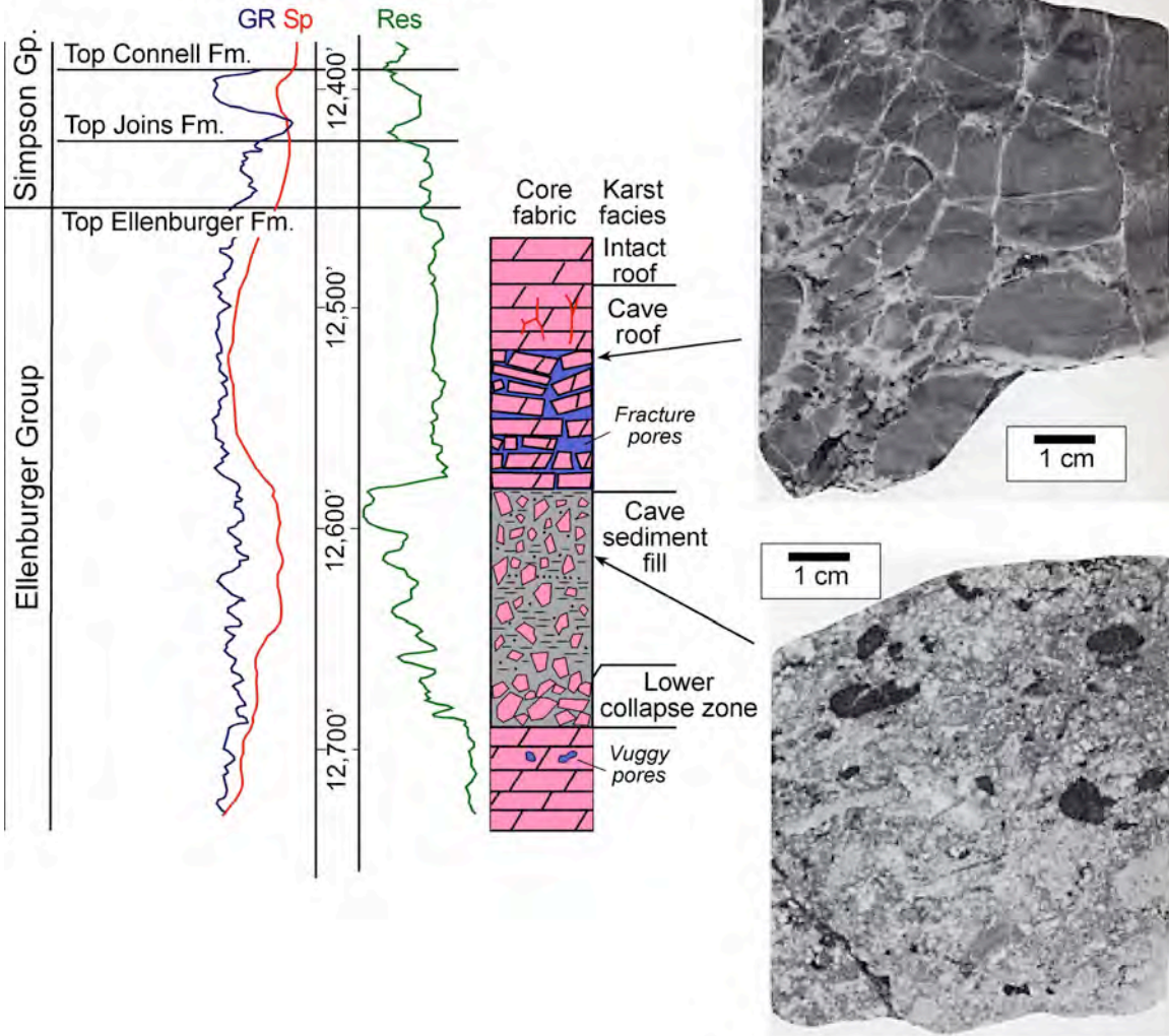
Figure 28. Core and wireline logs from the Gulf #000-1 TXL, Emma reservoir (Andrews County, Texas). Upper photograph from 12,526 ft shows crackle-fracture pores in collapse cave roof. Lower photograph from 12,610 ft shows cave-sediment fill (debris flow) with clasts floating in matrix of chloritic shale and quartz sand. From Kerans (1989).
