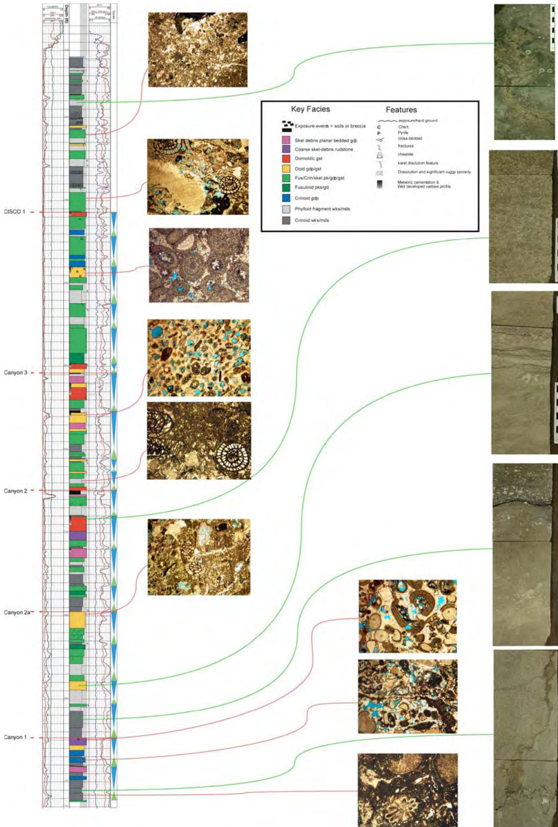
Figure 55. Type well log and facies for crestal grain-rich succession at SACROC. Note numerous transgressive and regressive cycles in green and blue. Core photos and photomicrographs both illustrate facies variability and differences in pore type, as well as potential permeability.
