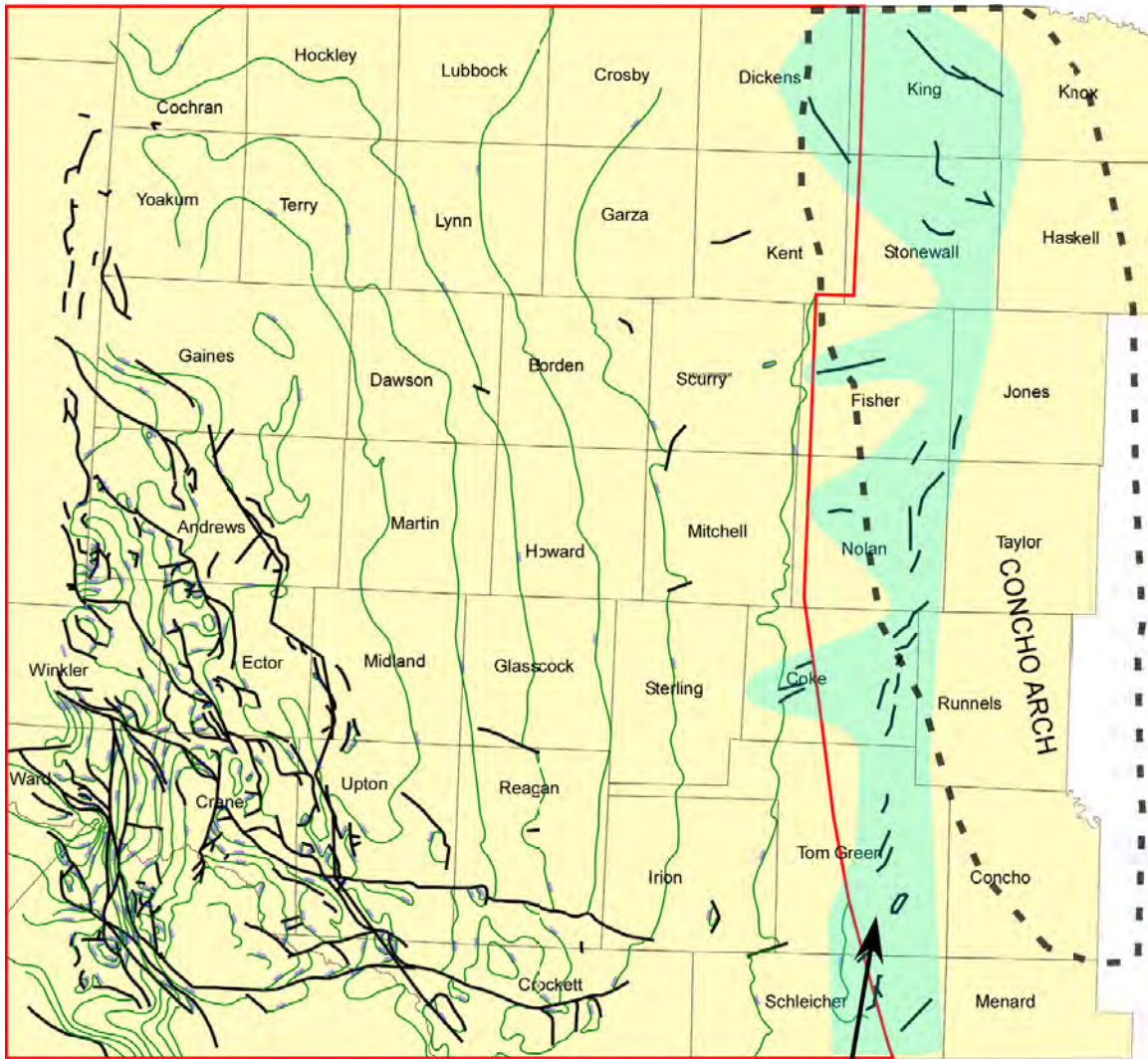
FORT CHADBOURNE FAULT ZONE
