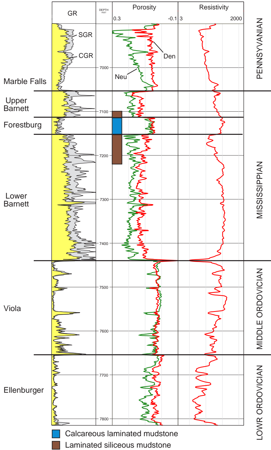
Figure 16. Typical wireline log signature of the Barnett Formation in the Ft. Worth Basin.
