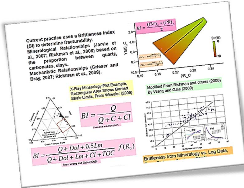
Figure 6. Various mineralogic indices for so-called brittleness prediction.
