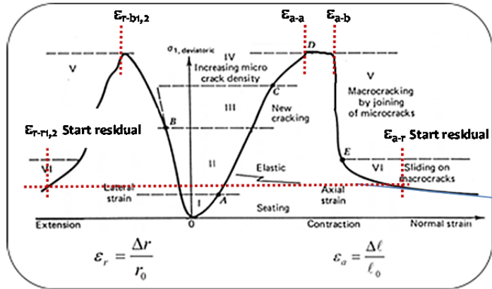
Ratio of Stable Plastic Strain to Strain at Residual (axial)
