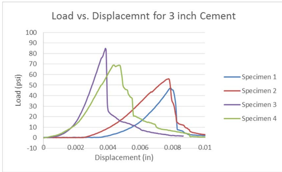
Figure 4. Load versus displacement for 3-inch cement samples.
