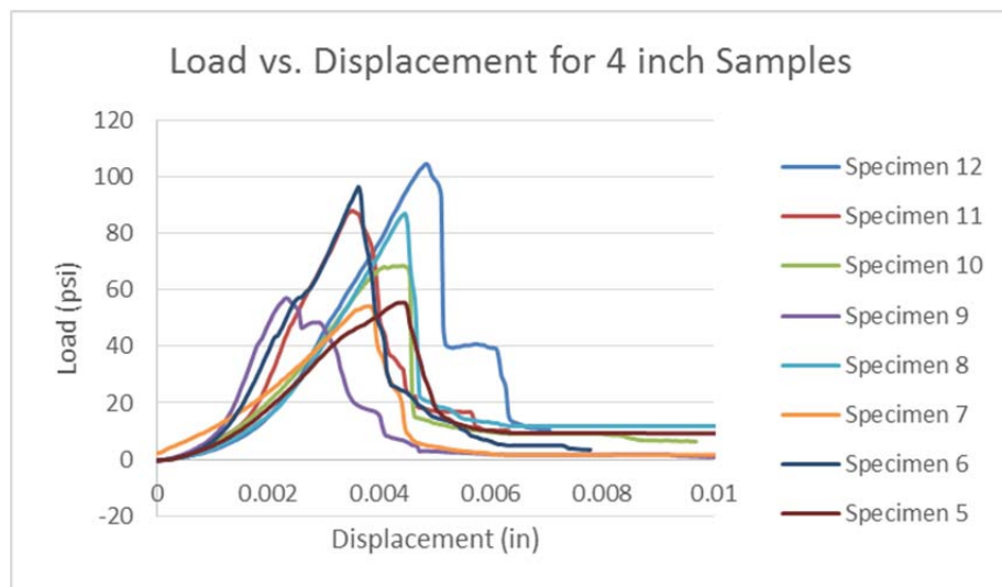
Figure 5. Load versus displacement for 4-inch cement samples.
