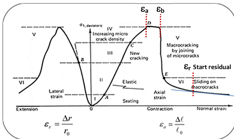
Ratio of Stable Plastic Strain to Strain at Residual (axial)
