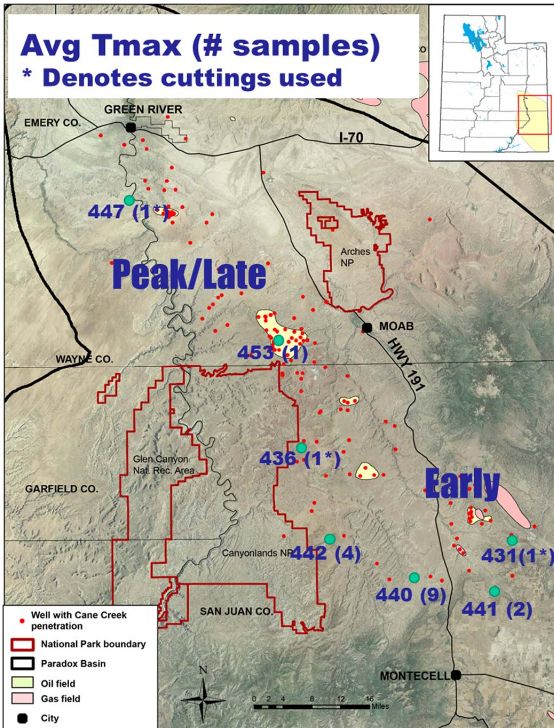
Figure 6. Average Tmax values from Cane Creek cores and cuttings indicate that areas to the south might be in the early oil generation window, whereas areas further north are in the peak to late oil generation window. This may help explain why production in the central portion of the play has been more successful than in the southern areas.
