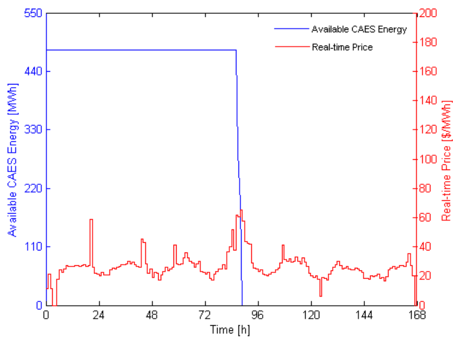
Exhibit 46 CAES Optimal Schedule with Natural Gas (Energy)
