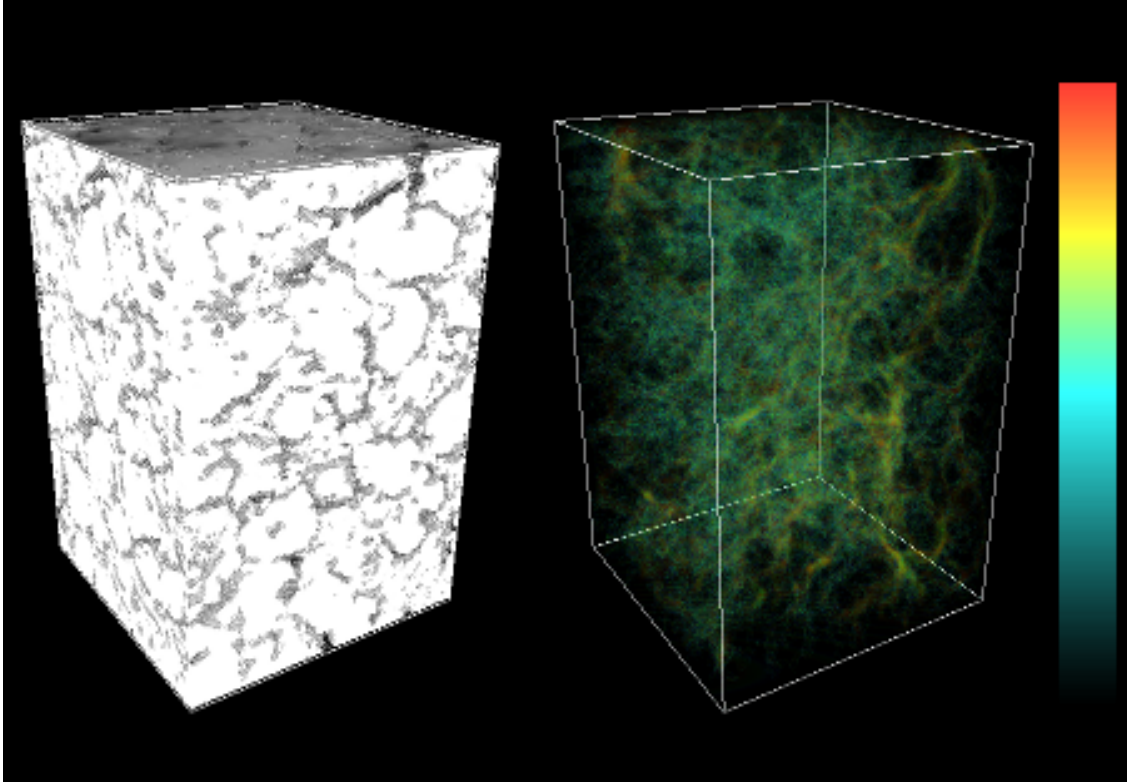
Figure 16. 3D views of LB simulated flow through the reconstructed XNT image of region A of the oil shale pyrolysis product prepared at 400^{\circ}\text{C} . Left: solid phase as white. Right: transparent solid phase to reveal flow channels. The estimated permeability is 0.000363 \mu\text{m}^2 or 0.363 \text{ mD} .
