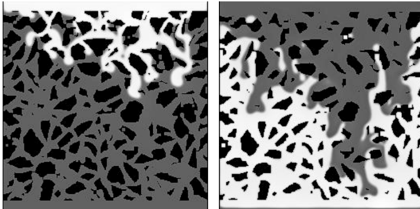
Figure 23. Two different penetration simulations for the same surface tension but inverse density ratio. Left: density ratio =3/1 and Ca = 6.77 \times 10^{-2} . Right: density ratio =1/3 and Ca = 1.32 \times 10^{-1} . Both images after 10,000 iterations.
