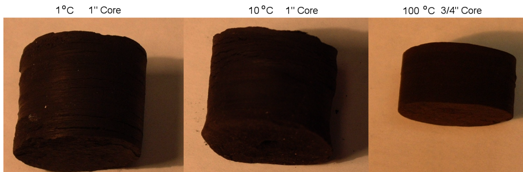
Figure 9. Reaction cores subjected to different heating rates (1, 10 and 100°C/min) prior to HRXMT analysis. The center reaction core has a drill hole at the central region of the core for insertion of the thermocouple wire.
