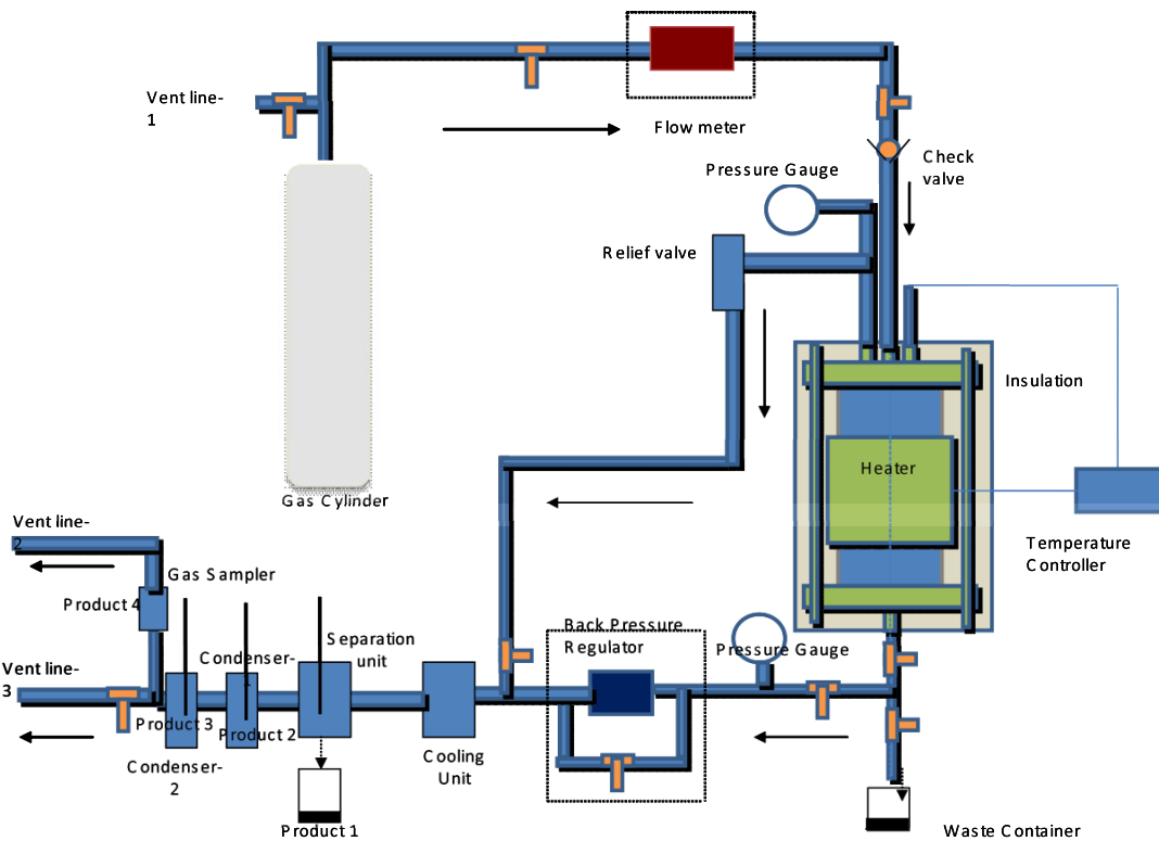
Figure 1. Schematic of the pyrolysis experiment for oil shale drill core samples.
