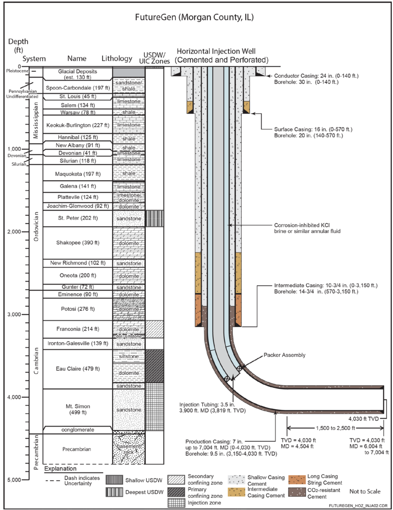
Figure 2-24. Proposed Horizontal Injection Well Construction Details
