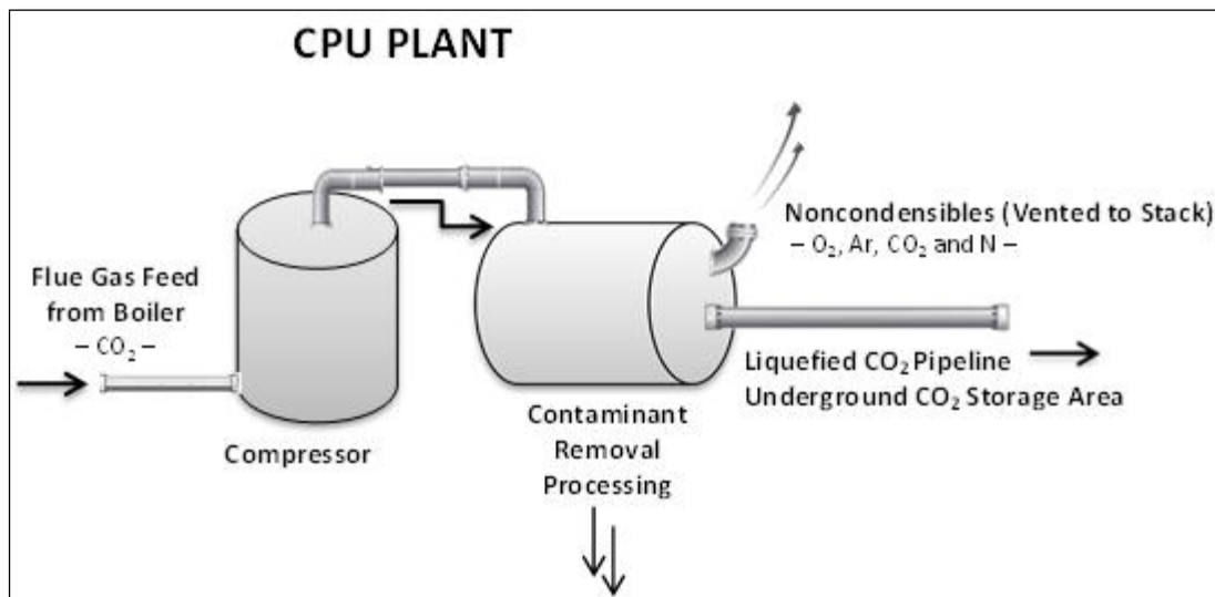
Figure 2-11. Basic Compression and Purification Process
